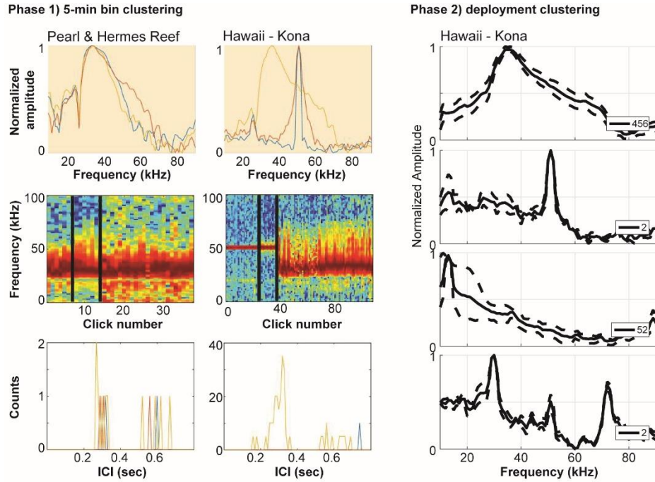
Figure 2. Examples for clustering phases 1 (5-min bin, click-based, left) and 2 (spectral average- and ICI mode-based, right). Phase 1 at Pearl and Hermes Reef: 3 Blainville’s beaked whale (Md) FM pulse spectral averages (top), concatenated spectra of all FM pulses in these averages (middle) and corresponding ICI distribution (bottom); Hawaii-Kona: 2 clusters of echosounders and one cluster of FM pulses. Phase 2 (Hawaii, 1 deployment): most 5-min bin spectral averages and ICI modes were clustered within the Md FM pulse type while several different echosounder categories occurred as well (additional not shown).
