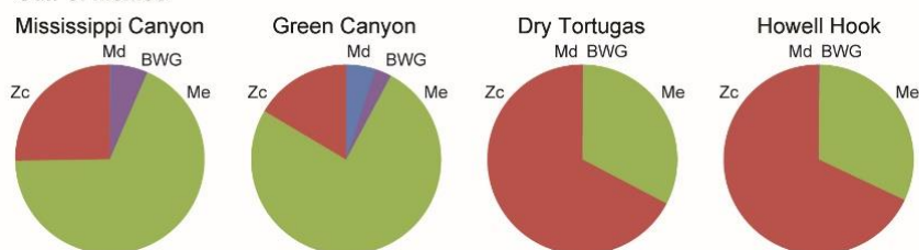
Figure 3. Relative presence of all beaked whale species at sites with Md pulse type detections based on cumulative minutes of acoustic encounters.
