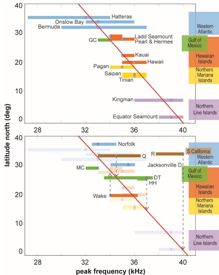
Figure 5. Increasing peak frequency (median with 25 th and 75 th percentiles) with lower latitudes (red regression line; y = -4.8x + 191.7 , R^2 = 0.93 ) at sites with regular Blainville's beaked whale presence (top). Sites with low numbers of detections (<1% of recorded days) may indicate transient whales from other regions (arrows, bottom).
