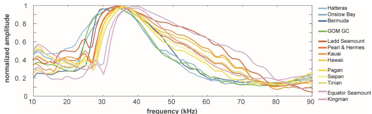
Figure 4. Spectral averages of primary cluster at sites with regularly occurring Md pulse type detections.
