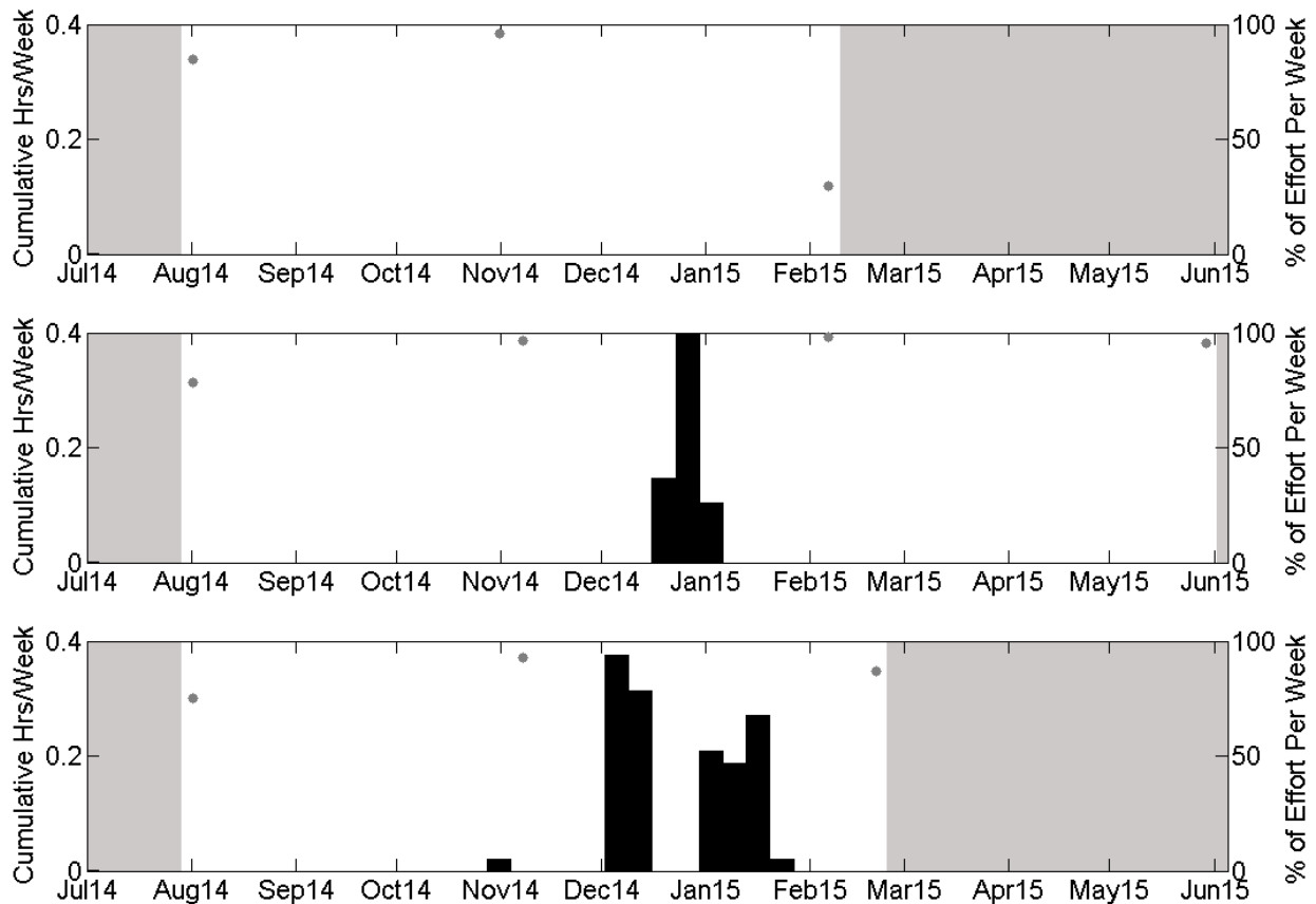
Figure 16. Weekly presence of BW43 FM pulses between July 2014 and May 2015 at sites M (top), H (middle), and N (bottom). Effort markings are described in Figure 11.
