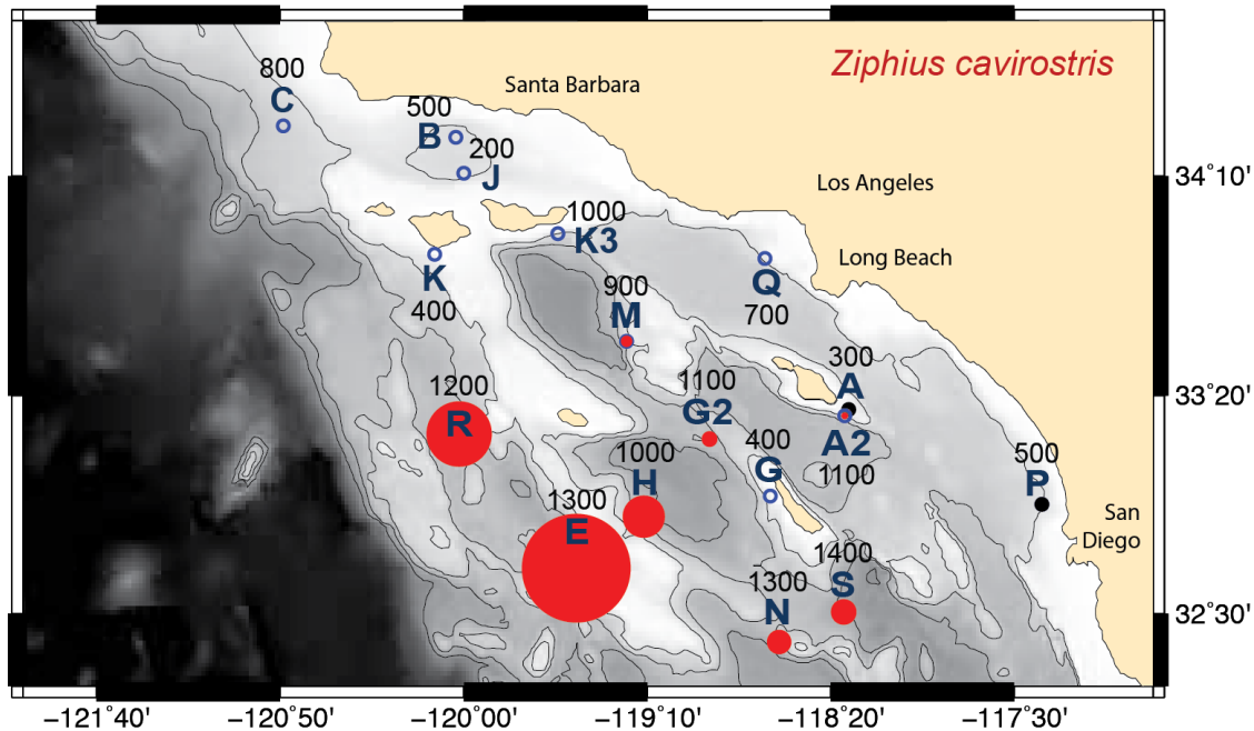
Figure 9. Relative density, based on total acoustic encounter durations normalized by effort, for Cuvier's beaked whales in the Southern California Bight. The circle size by each site gives the proportion of time bins with detections divided by the amount of time monitored. Site E with the largest circle had 45 minutes of average daily acoustic detections. The number above each site gives approximate bathymetric depth in meters. Preliminary results after Baumann-Pickering et al. (2015), data analysis continuing.
