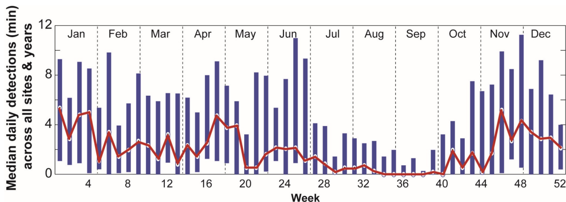
Figure 3. Seasonal trend of Cuvier's beaked whale presence in the Southern California region, from Baumann-Pickering et al. (2015). Blue bars show median and 1 st and 3 rd percentiles, red line follows median.
