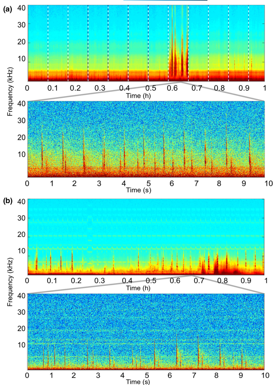
FIGURE 2 Sperm whale clicks from Guys Bight (a) recorded on September 23, 2015 and from Pond Inlet (b) recorded on August 8, 2019. The top panel from each site displays a long-term spectral average (LTSA) and the bottom panel displays the spectrogram. The Guys Bight LTSA (a) has vertical lines delineating gaps in the data as a result of the duty cycle. So although the LTSA displays 1 h of acoustic data, the overall length of the data shown encompasses 12 h
