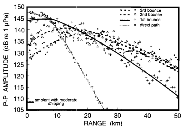
FIG. 3. The amplitude of an airgun source versus range for the direct water path and bounce paths as received on a seafloor recorder during this study.
