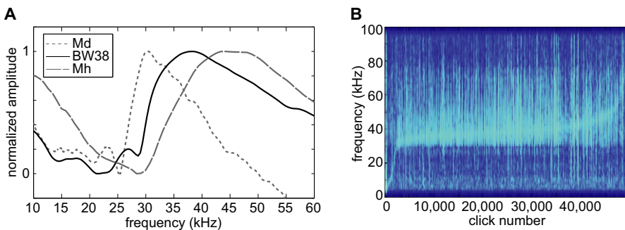
Figure 2. Characteristics of the beaked whale frequency-modulated (FM) pulse type of unknown origin, named BW38, based on peak frequency. (A) Mean spectra of BW38 FM pulse type (bold black line) in comparison to mean spectra of FM pulses produced by Blainville's beaked whales (Md) and Deraniyagala's beaked whales (Mh) (Baumann-Pickering et al. 2013a). (B) Concatenated spectrogram of all BW38 FM pulses sorted by peak frequency.
