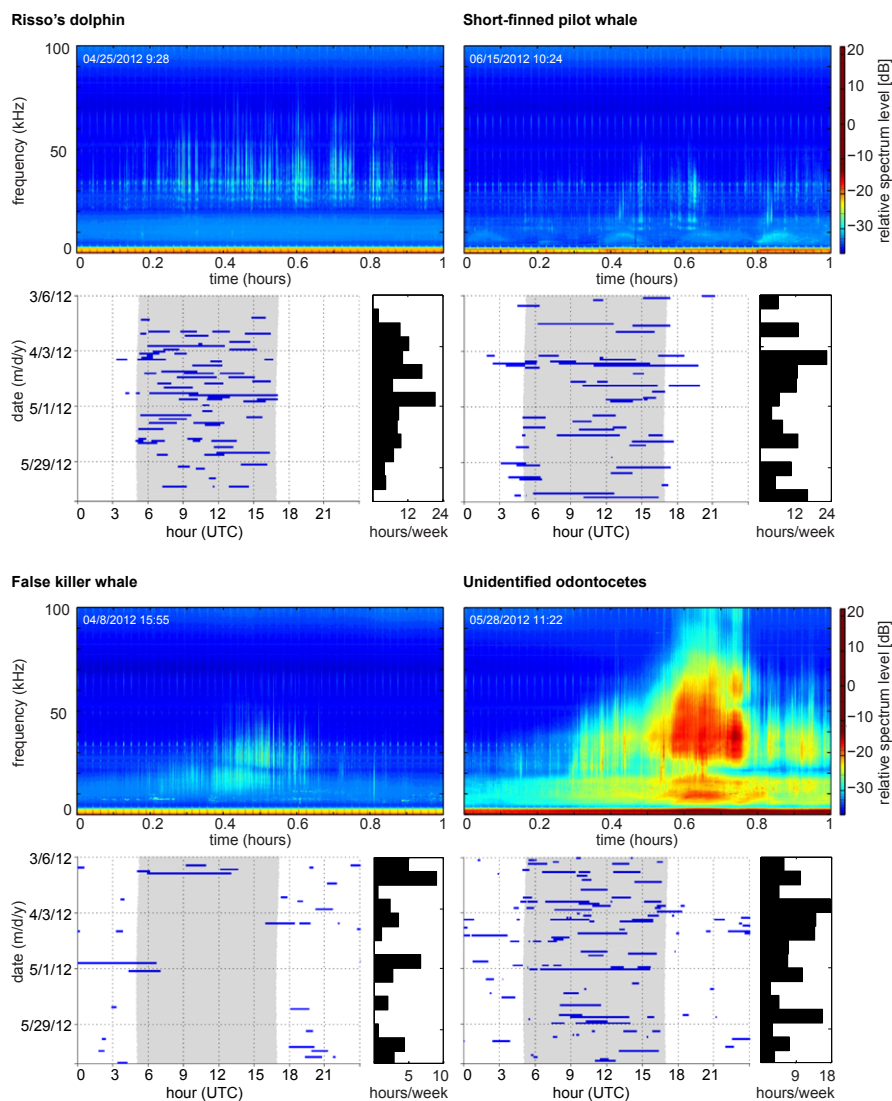
Figure 4. Acoustic encounters of Risso's dolphins (top left), short-finned pilot whales (top right), false killer whales (bottom left), and unidentified odontocetes (bottom right). Long-term spectral average examples (top) and diel and weekly occurrence (bottom) are shown for each species or group.
