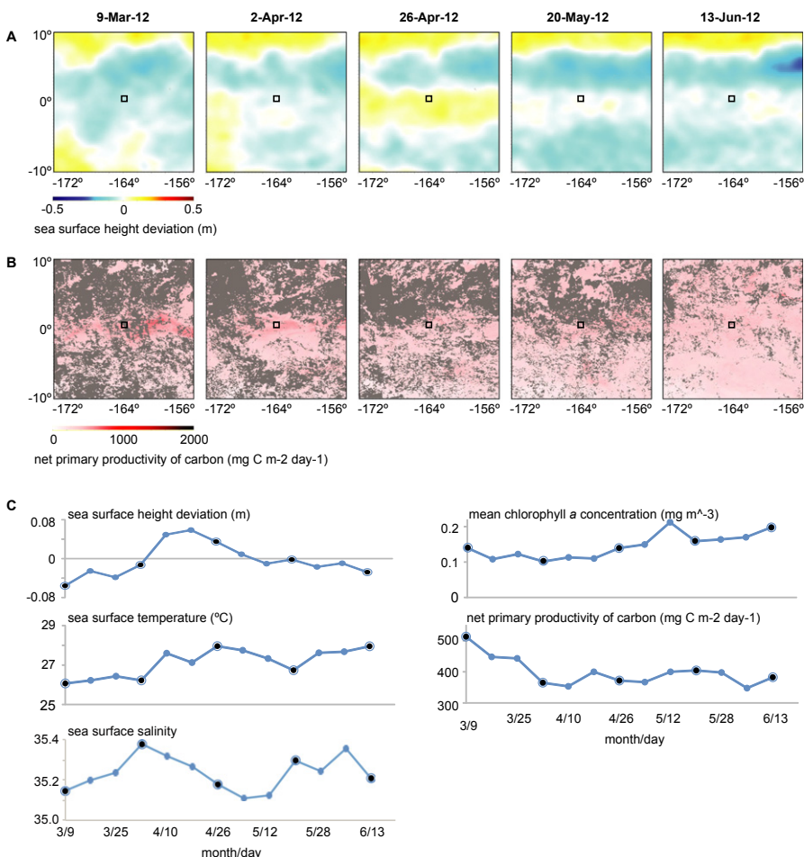
Figure 6. Oceanographic changes in the broader area surrounding the study site during the recording period of the HARP using 8 d composite remotely sensed data. (A) Sea surface height deviation and (B) net primary productivity of carbon over 10°N to 10°S and 174°W to 154°W. (C) Progression of 8 d composite values for sea surface height deviation, mean chlorophyll a concentration, sea surface temperature, net primary productivity of carbon, and sea surface salinity over time taken from a 20 km × 20 km area (black square in A and B, not to scale) centered on the HARP location.
