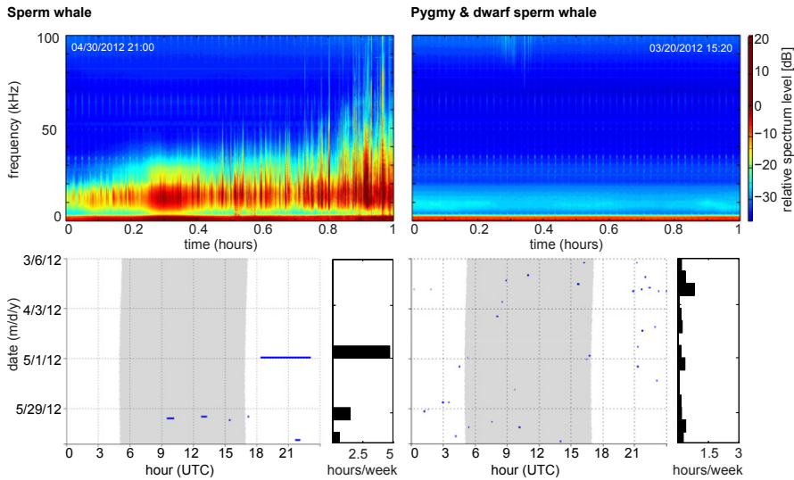
Figure 5. Acoustic encounters of sperm whales (left) and Kogiidae (pygmy and dwarf sperm whales, right). Long-term spectral average examples (top) and diel and weekly occurrence (bottom).
