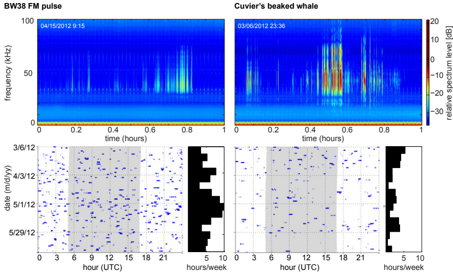
Figure 3. Acoustic encounters of BW38 FM pulse type (unknown origin, left) and Cuvier's beaked whales (right). Long-term spectral average examples (top) and diel and weekly occurrence (bottom).
