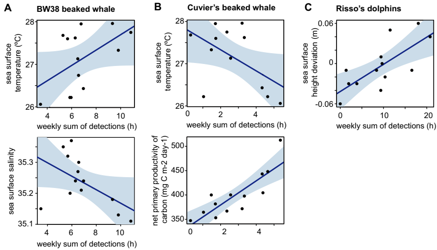
Figure 7. Linear regression (line) of oceanographic variables and weekly hours of acoustic detections of species or signal type (points) with 95% confidence intervals (shading).
