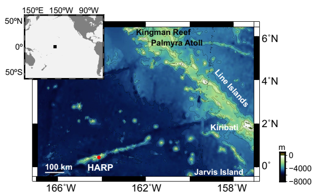
Figure 1. Location of HARP (square: top left) in central equatorial Pacific. Bathymetric detail (HARP as red circle at 1,300 m depth) at an unnamed seamount chain near the equator in the vicinity of the Northern Line Islands, nearly due south of Kingman Reef and Palmyra Atoll. Few bathymetric features exist further south and west of the HARP location.
