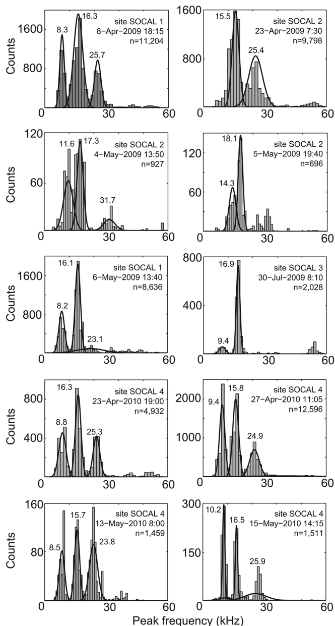
FIG. 3. Peak frequency distribution of echolocation signals in ten individual HARP encounters (site, date, time, and n number of echolocation signals given). GMM with five mixtures fitted (line) to the peak frequency histogram, probability of fit was omitted, and only dominant fits are shown to simplify graphs.
