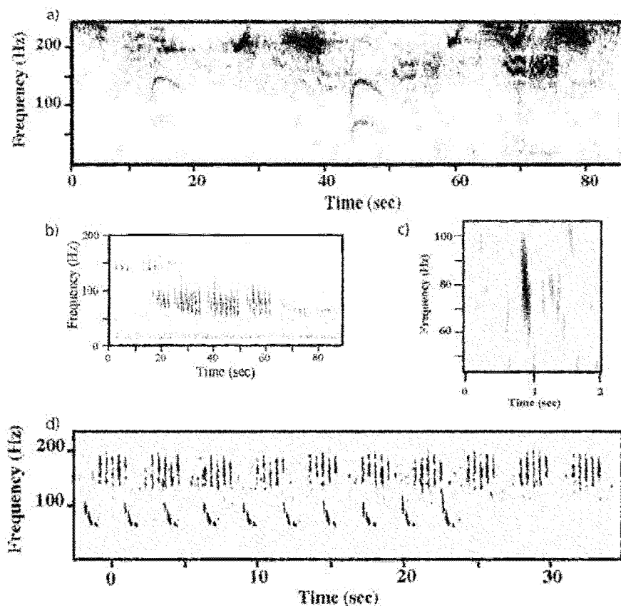
Figure 6.1. Spectrograms of calls of other marine mammals recorded on the ARPs deployed off the Western Antarctic Peninsula: a) crabeater seal; b) humpback whale; c) minke whale; and d) unknown calls.
