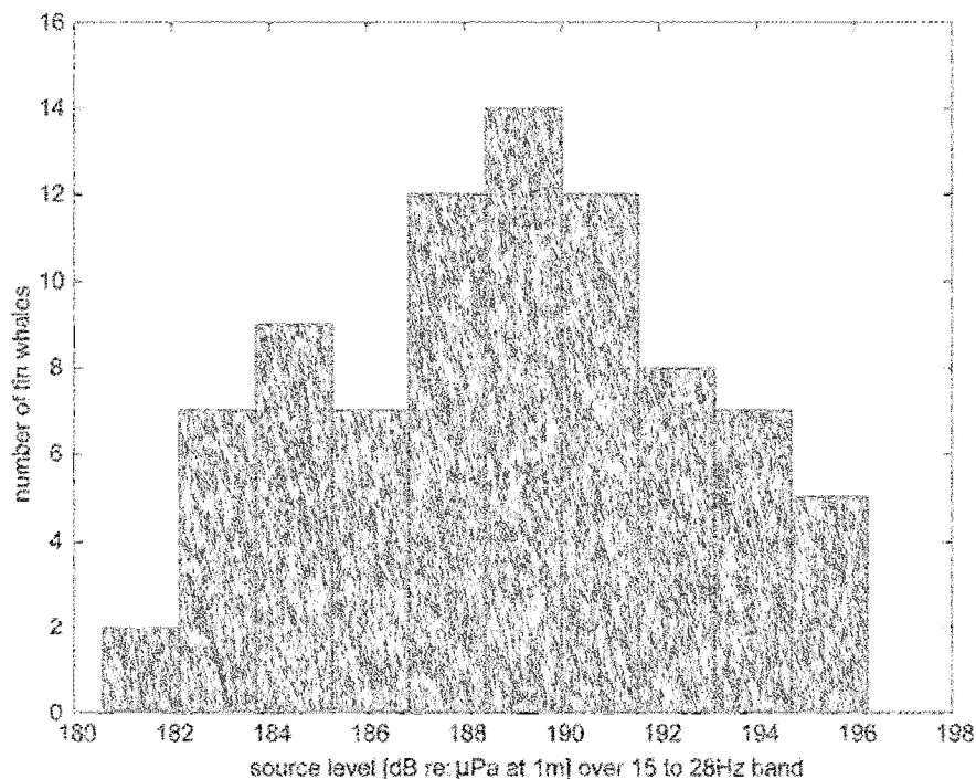
Figure 3.7. Distribution of fin whale call source levels (N=83).
