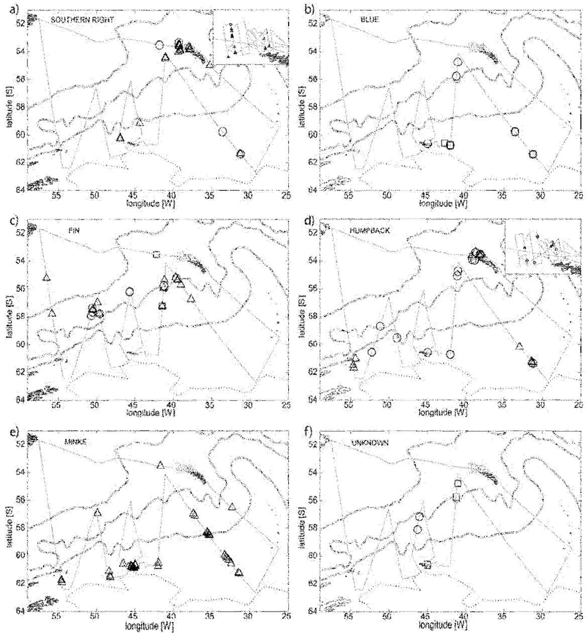
Figure 5.3. Locations of acoustic (circles and squares) and visual (triangle) sightings: a) southern right; b) blue (circles are tonal call and squares D call locations); c) fin (circles are low frequency and squares high frequency call locations); d) humpback; e) minke whales. f) Locations of 50Hz up (circles) and pulsing calls (squares). Insets on a) and d) show sightings in the WCB. Thin grey line is the cruise track, thick grey lines represent major fronts in the area: PF; sACCf; SB and the broken black line is the inferred ice edge on 1 February 2003 from the NSIDC satellite image (same as Figure 1).
