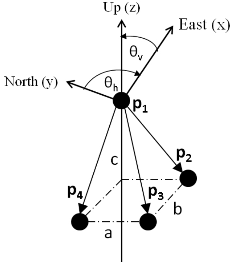
Figure 4.2. Schematic of the volumetric small-aperture array defined by its four hydrophone position vectors \mathbf{p}_1, \dots, \mathbf{p}_4 with spacing a = 0.9 \text{ m} , b = 1.1 \text{ m} and c = 0.9 \text{ m} . y and x axis are aligned with the northern and eastern cardinal direction. Horizontal angles, \theta_h , are measured clockwise with respect to the y -axis with 0^\circ corresponding to North. Vertical Angles, \theta_v , are ranging from -90^\circ (straight below \mathbf{p}_1 ) to +90^\circ (straight above \mathbf{p}_1 ).
