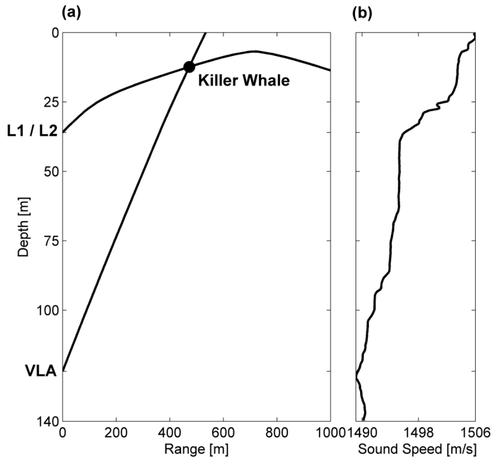
Figure 2.4. Range and depth estimation. Intersection of rays (a) provides a range and depth estimate for a clicking killer whale (black circle). The vertical arrival angles at the L-shaped arrays and VLA were used as start angles for two rays, which were back-propagated using the measured sound velocity profile (b) to account for refraction.
