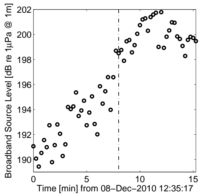
Figure 4.5. Broadband source level as a function of time for ship track (a) of Figure 4.3. Dashed line indicates the time of the CPA with a slant range of 1.29 km to the volumetric seafloor array.
