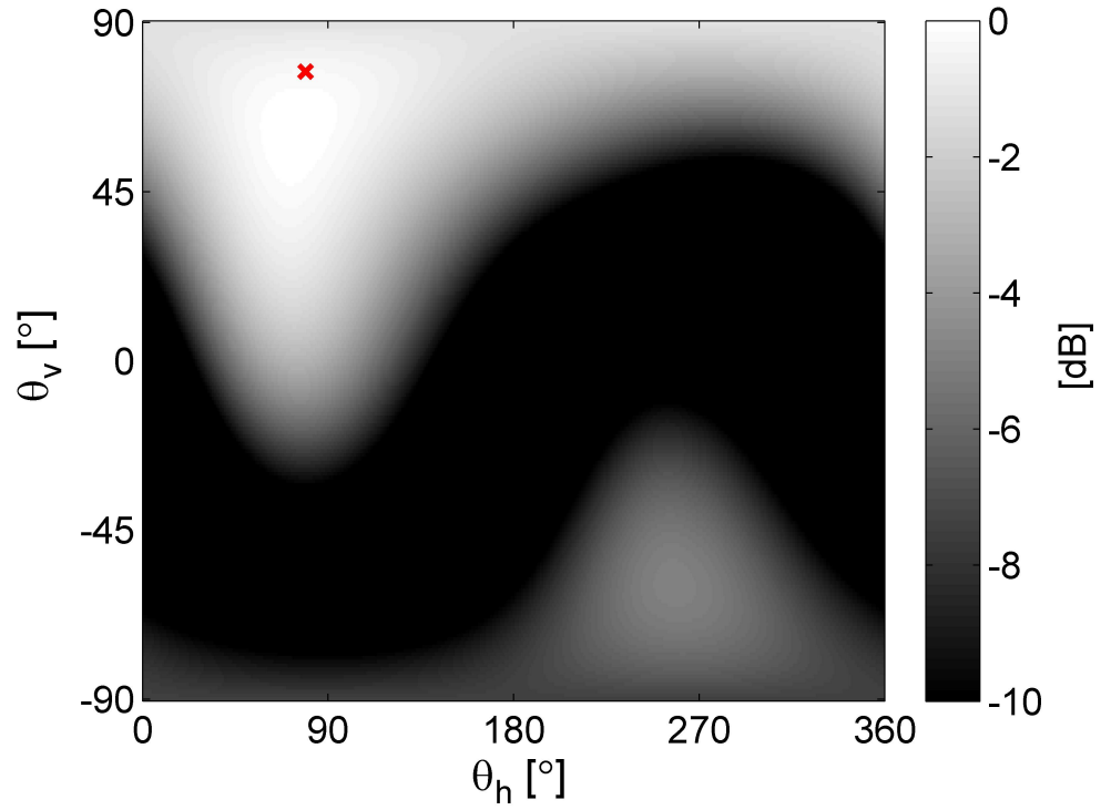
Figure 4.7. Beampattern of the frequency domain beamformer (FDB) at the CPA of ship track (a) from Figure 4.3 for a frequency of 410 Hz . The FDB beampattern was normalized by its maximum for all vertical and horizontal angles, \theta_v and \theta_h , respectively, and is shown for a dynamic range of 10 dB (greyscale colormap). The beampattern peaks at \theta_{v_s} = 77^\circ and \theta_{h_s} = 79^\circ as indicated by the red cross.
