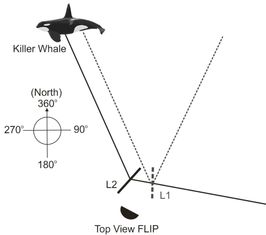
Figure 2.5. Bearing estimation. Bearings of the horizontal components for the L1 and L2 arrays are represented by the dashed line and the solid line, respectively. Each array measures two possible bearings due to the left-right ambiguity common to line arrays. This ambiguity is resolved by selecting the bearings that give consistent locations between L1 and L2.
