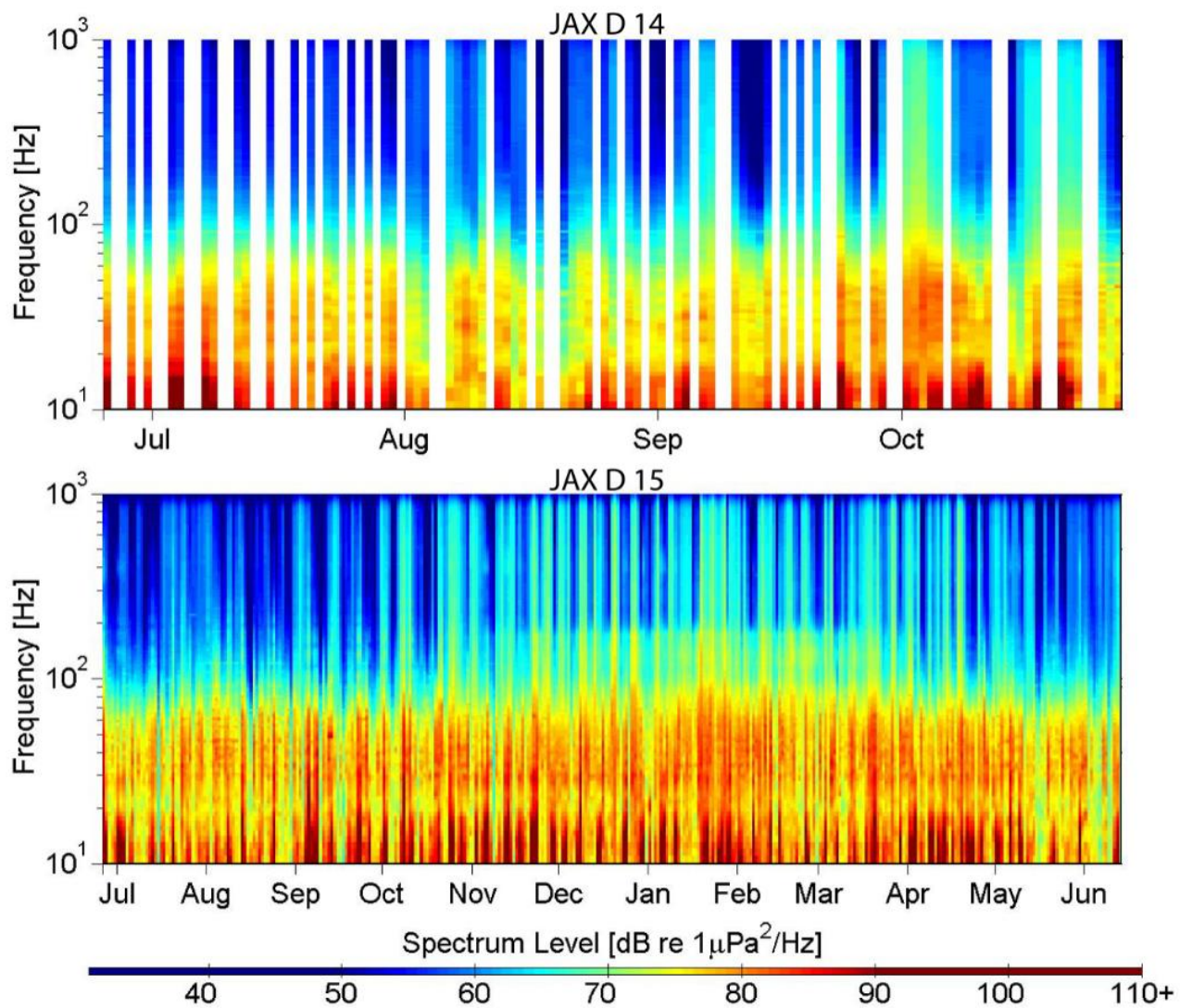
Figure 14. Long-term spectrograms using daily-averaged spectra for JAX Site D from June 2017 to 2019.
