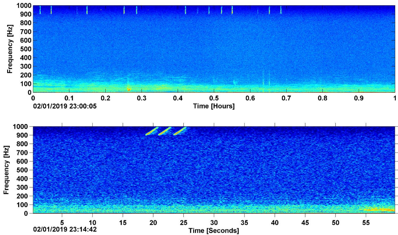
Figure 9. Low-Frequency Active (LFA) sonar in Hz in the LTSA (top) and spectrogram (bottom) recorded at JAX Site D, February 2019.
