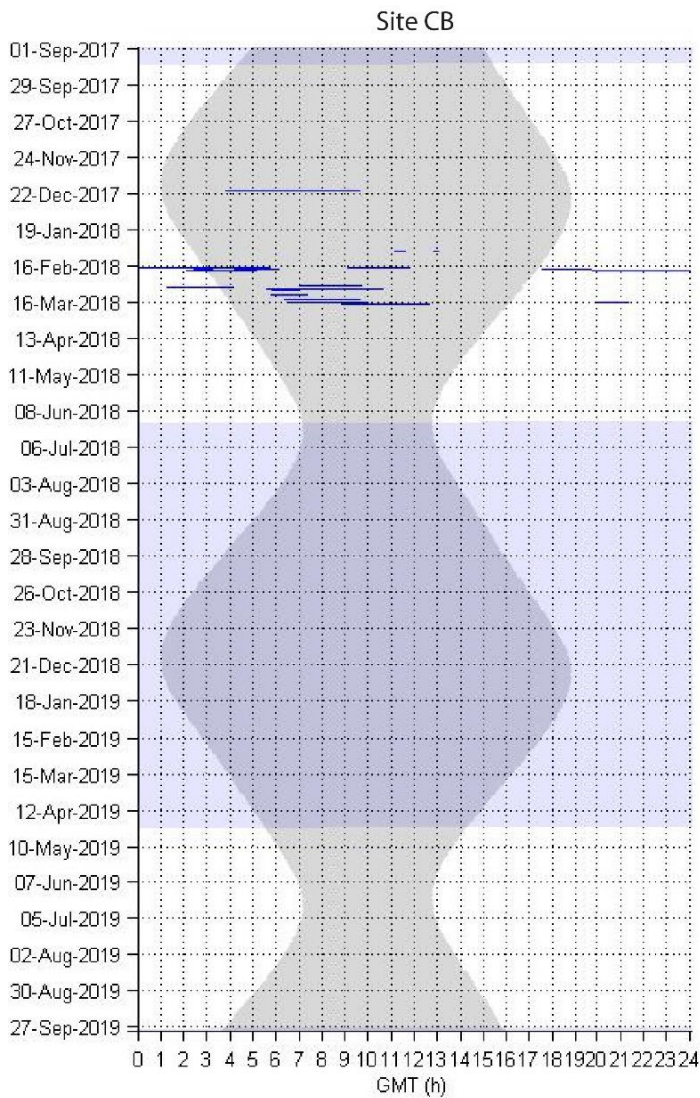
Figure 29. Diel presence of humpback whale calls, indicated by blue dots, in one-minute bins at sites CB (left) and KOA (right).
