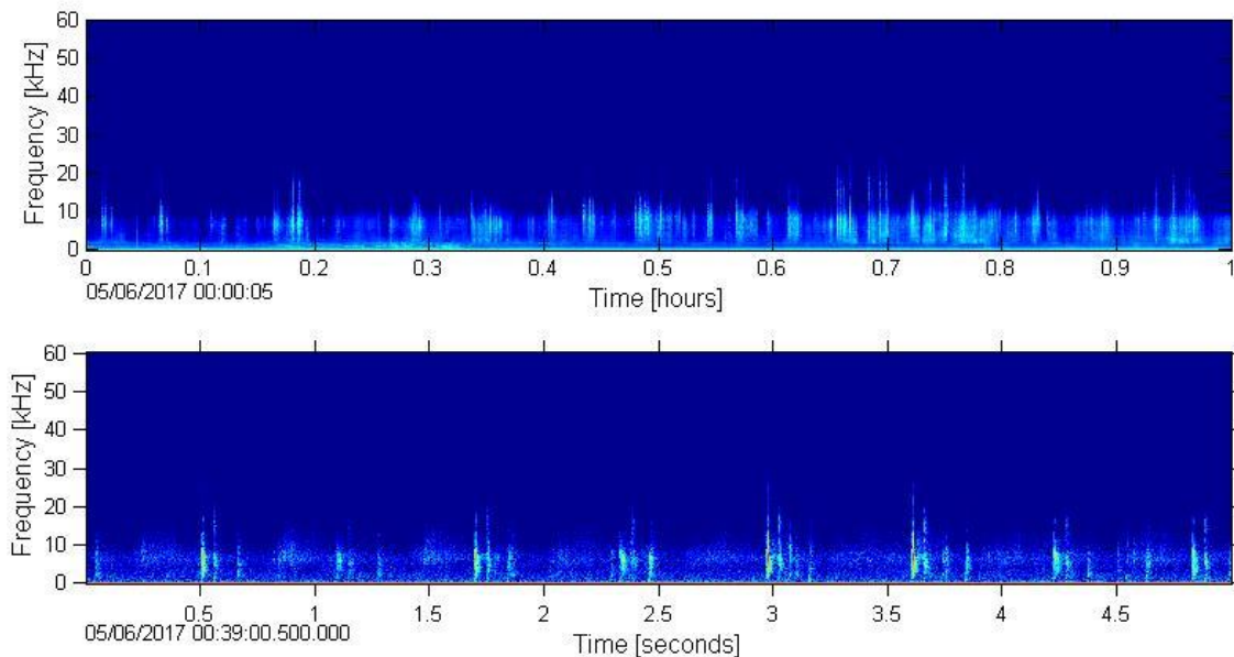
Figure 12. Sperm whale echolocation clicks in an LTSA (top) and spectrogram (bottom) recorded at site CB.
