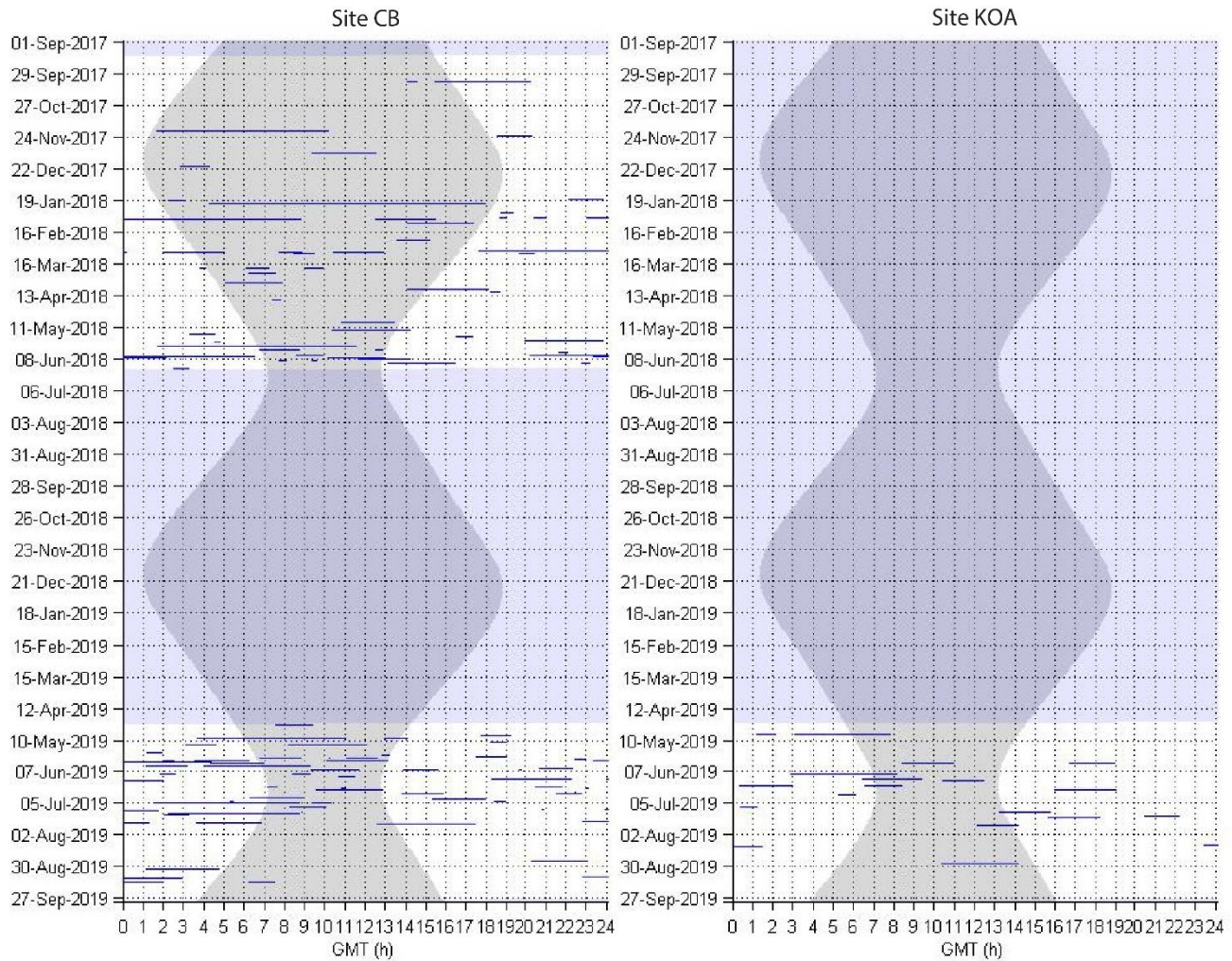
Figure 31. Diel presence of killer whale whistles and pulsed calls, indicated by blue dots, in one-minute bins at site CB (left) and KOA (right).
