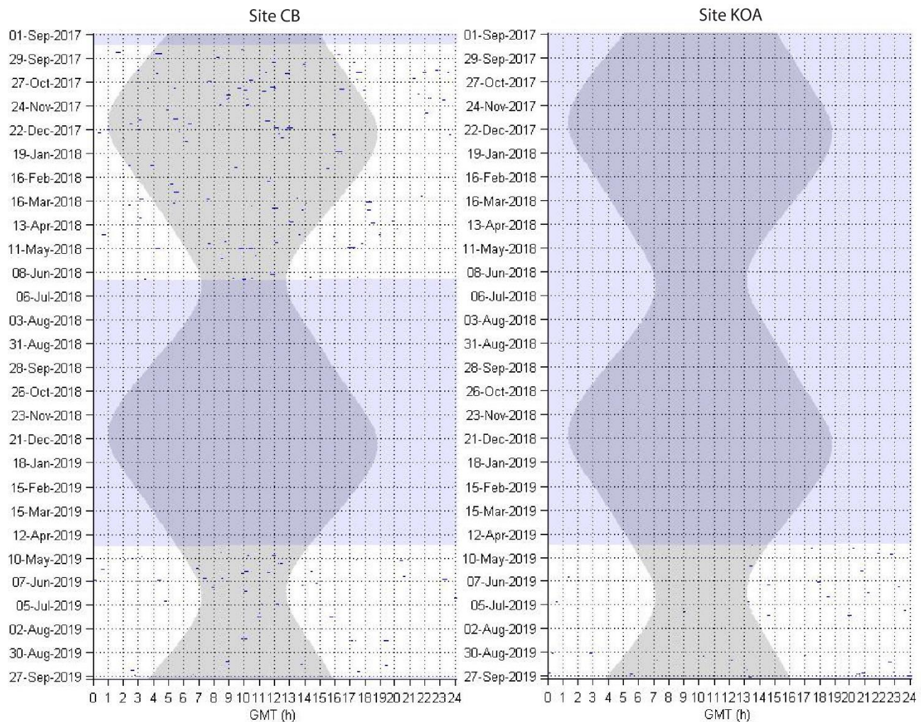
Figure 37. Diel presence of Stejneger's beaked whale FM pulses, indicated by blue dots, in five-minute bins at sites CB (left) and KOA (right).
