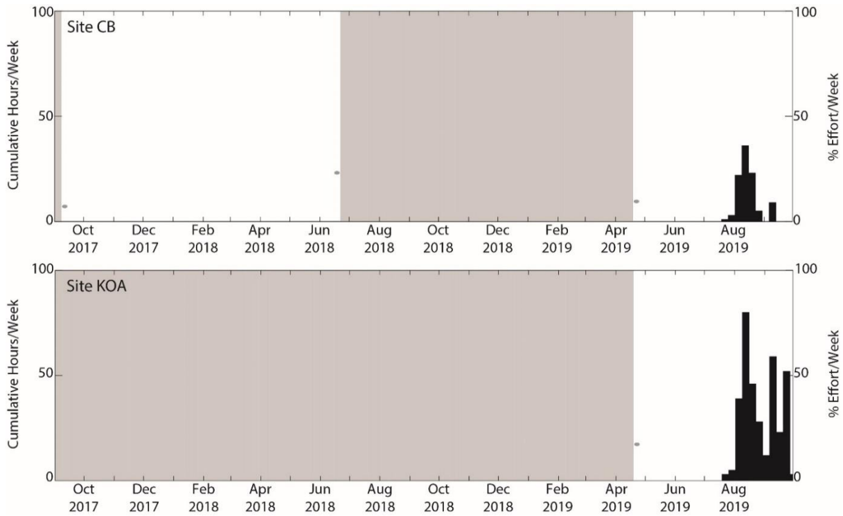
Figure 21. Weekly presence of Central Pacific tonal blue whale calls from September 2017 to June 2018 and April to September 2019 at sites CB (top) and KOA (bottom).
