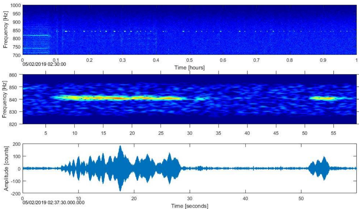
Figure 16. A tonal Low-frequency Active (LFA) sonar in an LTSA (top), spectrogram (middle), and timeseries (bottom) recorded at site CB.
