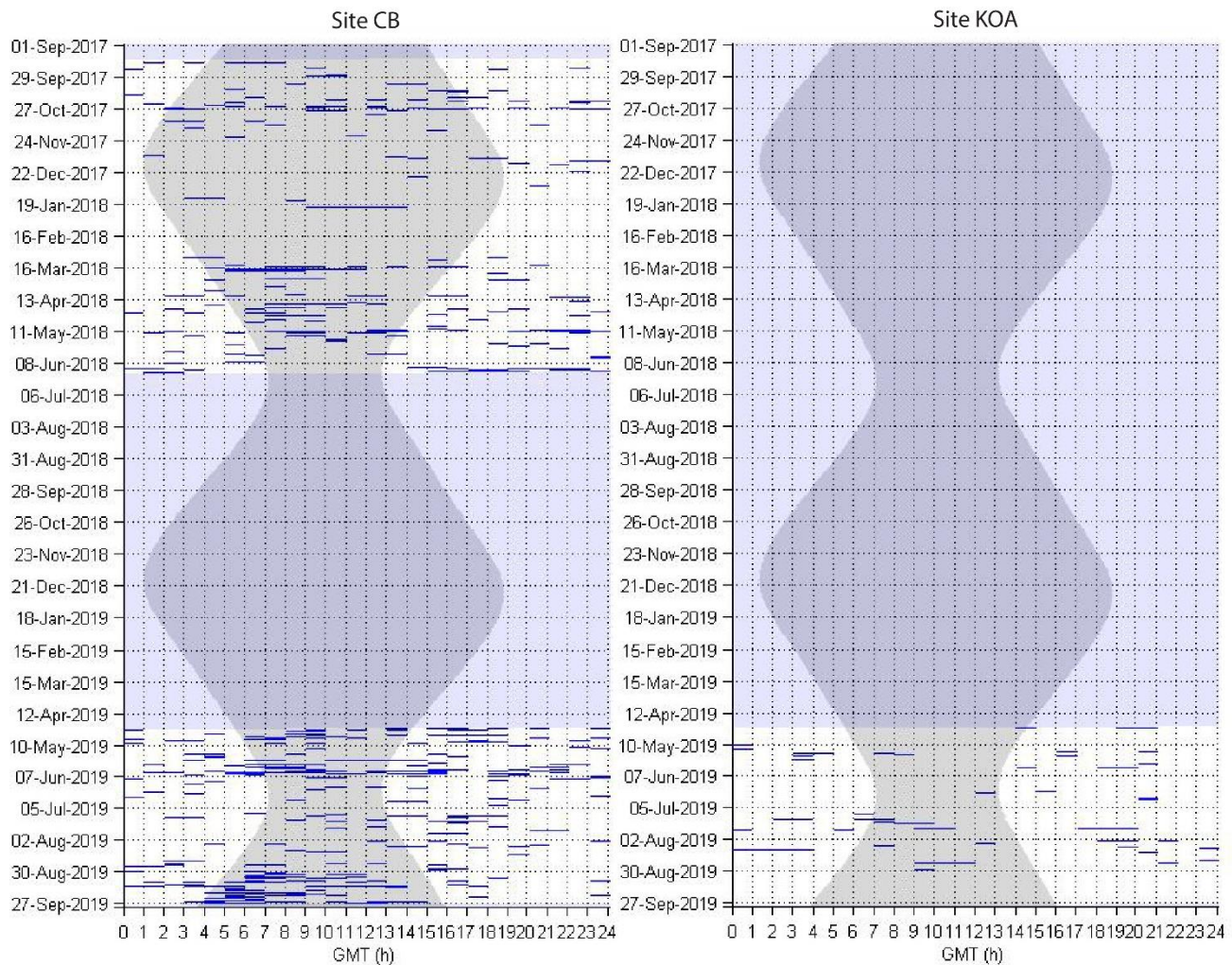
Figure 27. Diel presence of fin whale 40 Hz calls, indicated by blue dots, in one-hour bins at sites CB (left) and KOA (right). Gray vertical shading denotes nighttime and transparent blue horizontal shading denotes absence of acoustic data.
