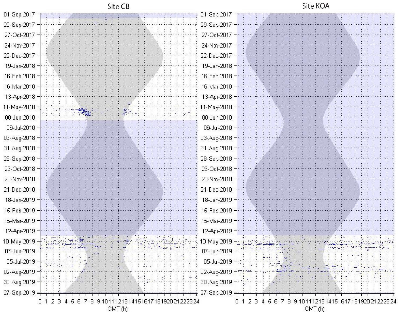
Figure 24. Diel presence of blue whale D calls, indicated by blue dots, in five-minute bins at sites CB (left) and KOA (right).
