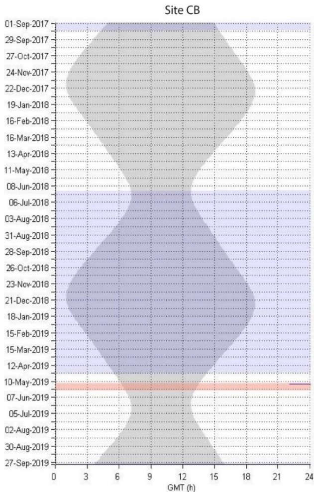
Figure 48. Major naval training events (shaded light red) overlaid on diel presence of LFA sonar < 500 Hz signals, indicated by blue dots, in one-minute bins at sites CB (left). There was no LFA sonar < 500 Hz detected at site KOA.
