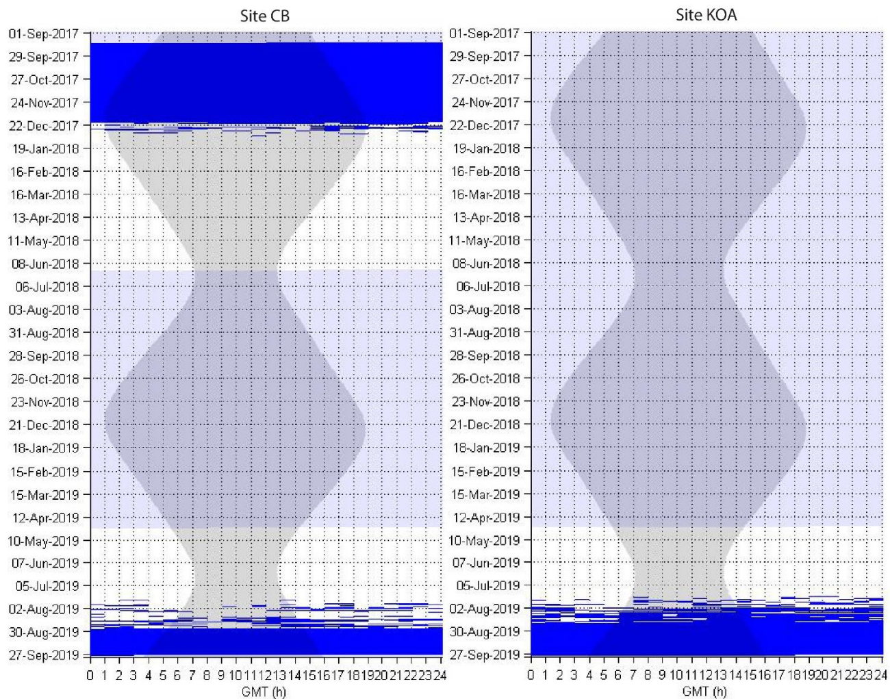
Figure 20. Diel presence of NE Pacific blue whale B calls, indicated by blue dots, in one-hour bins at sites CB (left) and KOA (right).
