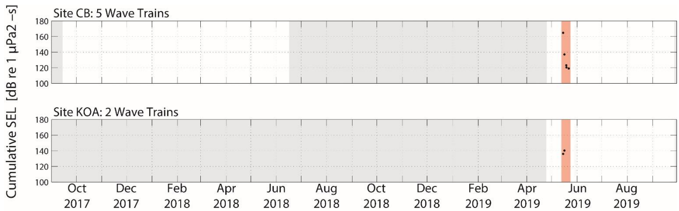
Figure 41. Cumulative sound exposure level for each wave train at site CB (top) and site KOA (bottom).
