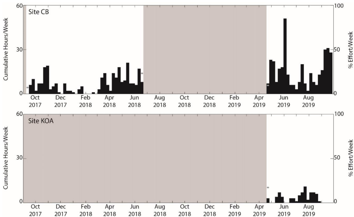
Figure 26. Weekly presence of fin whale 40 Hz calls from September 2017 to June 2018 and April to September 2019 at sites CB (top) and KOA (bottom). Gray dots represent the percent of effort per week in weeks with less than 100% recording effort, and gray shading represents periods with no recording effort. Where gray dots or shading are absent, full recording effort occurred for the entire week.
