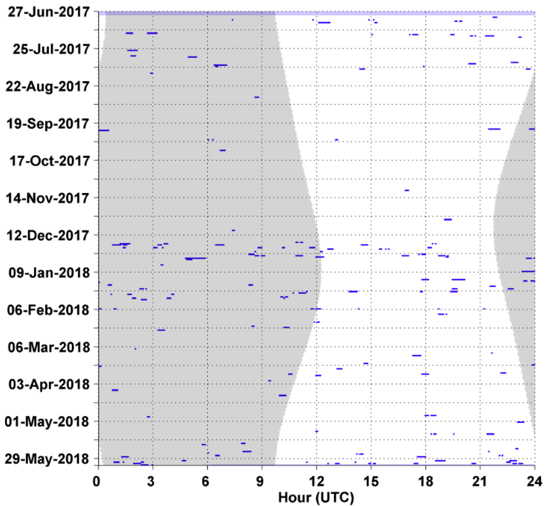
Figure 50. Cuvier's beaked whale echolocation clicks in one-minute bins at NFC Site A from June 2017 to 2018. Gray vertical shading denotes nighttime.
