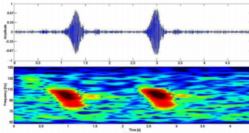
Figure 4. Waveform (top) and spectrogram (bottom) of Bryde's whale Be9 call from the Gulf of Mexico (Širović et al. , 2014).
