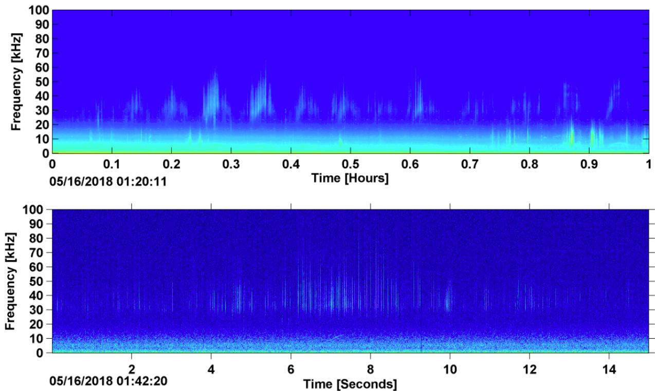
Figure 19. Click type CT 1 acoustic encounter in LTSA (top) and spectrogram (bottom) recorded at NFC Site A, May 2018.
