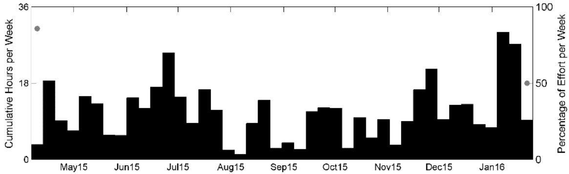
Figure 58. Weekly presence (black bars) of Click Type 1 detections from April 2015 to January 2016. Effort markings are described in Figure 41.
