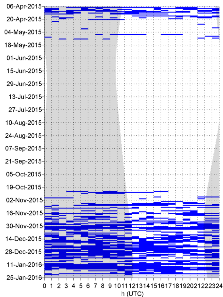
Figure 45. Minke whale pulse trains in hourly bins (blue bars) from April 2015 to January 2016. Effort markings are described in Figure 43.
