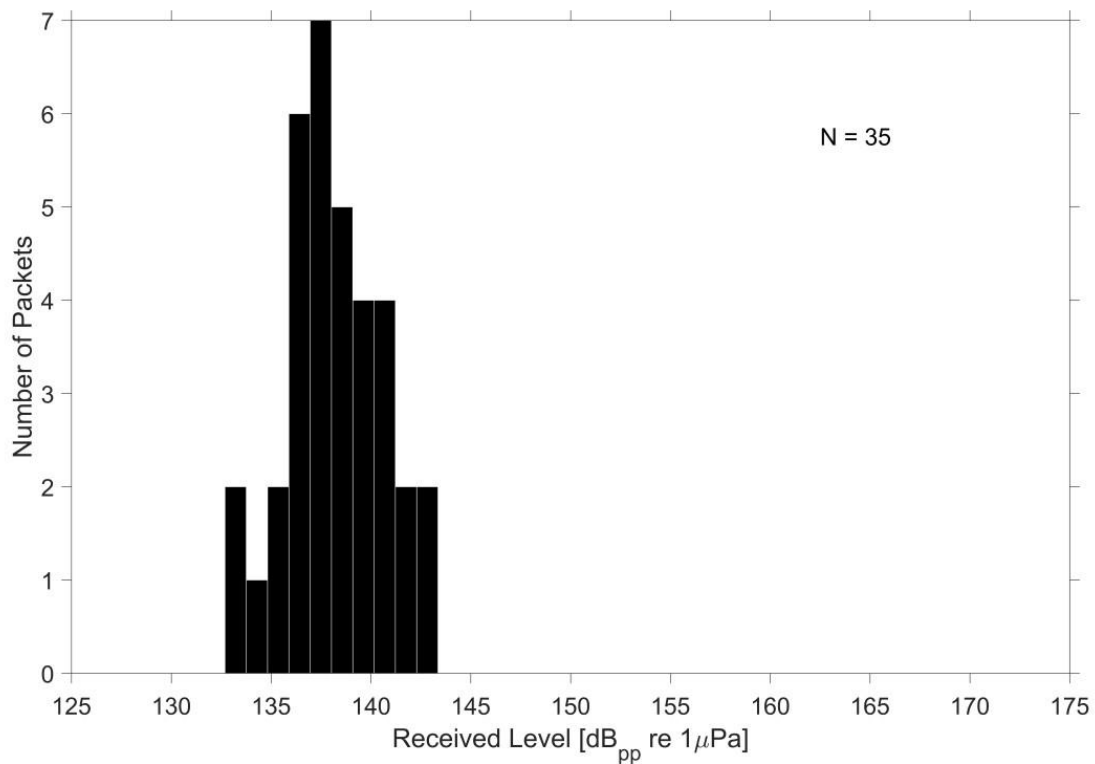
Figure 84. Distribution of received levels (dB pp re 1μPa) for MFA sonar in October 2015.
