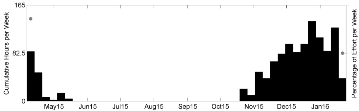
Figure 44. Weekly presence (black bars) of minke whale pulse trains from April 2015 to January 2016. Effort markings are described in Figure 41.
