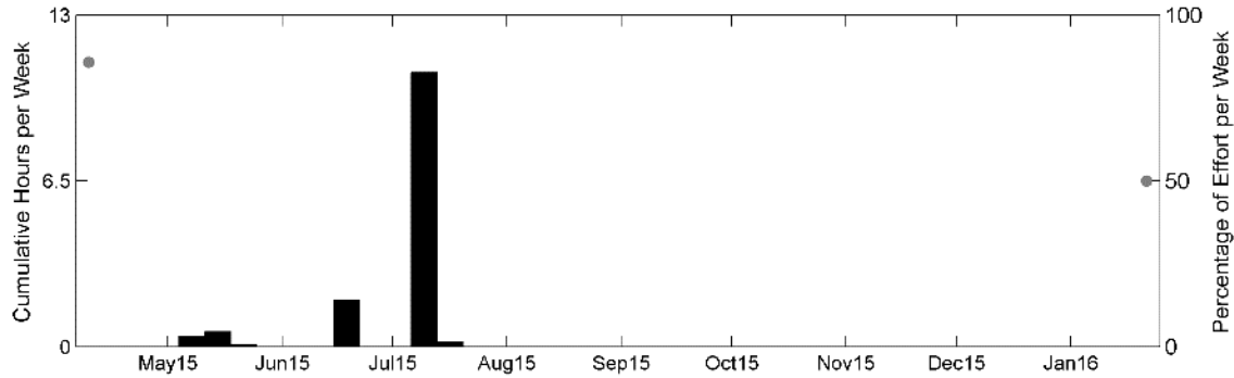
Figure 56. Weekly presence (black bars) of Risso's dolphin clicks from April 2015 to January 2016. Effort markings are described in Figure 41.
