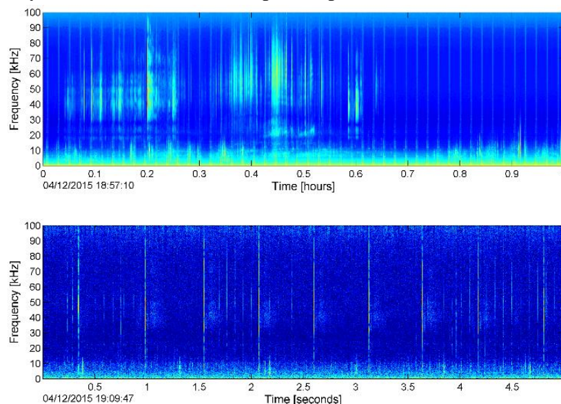
Figure 14. Cuvier's beaked whale echolocation clicks in LTSA (top) and spectrogram (bottom)
