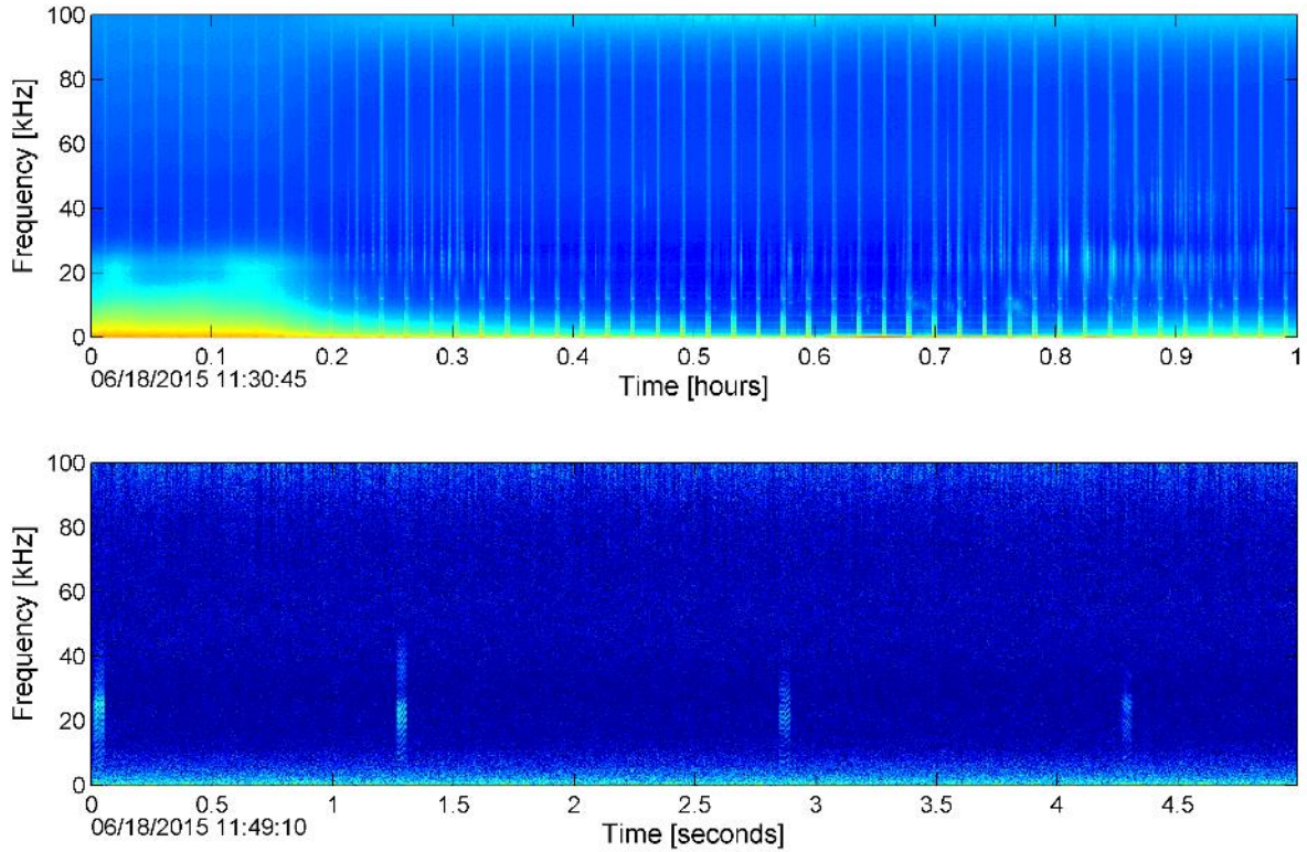
Figure 31. CT 7 in the LTSA (top) and spectrogram (bottom) recorded at HAT.
