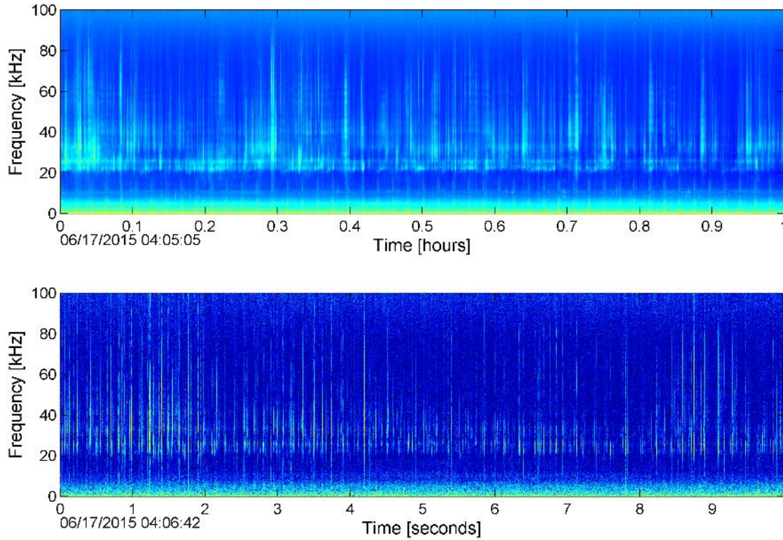
Figure 19. Risso's dolphin clicks in the LTSA (top) and spectrogram (bottom) at HAT.
