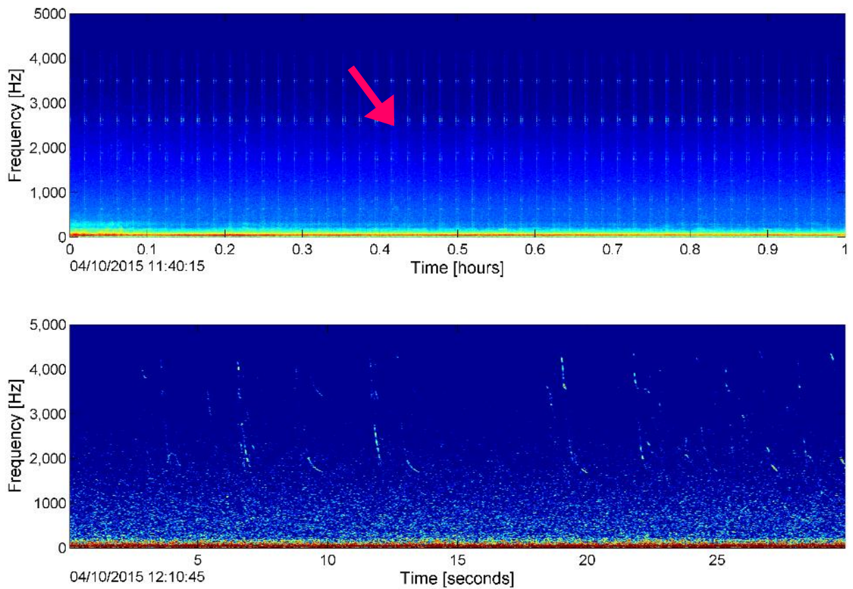
Figure 22. Unidentified odontocete whistles under 5 kHz in the LTS (top) and spectrogram (bottom) recorded at HAT. Red arrow indicates location of LTS expanded in the spectrogram.
