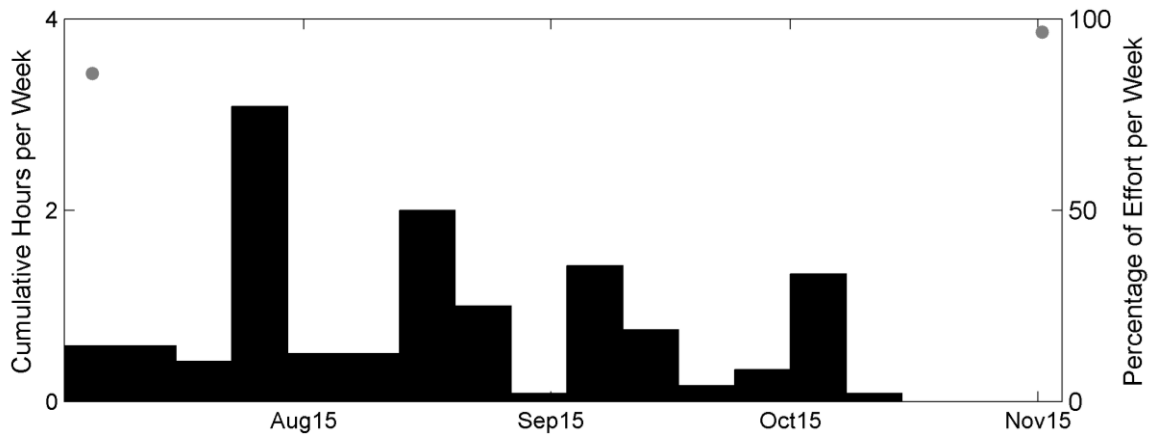
Figure 24. Weekly presence of unidentified odontocete clicks between July and November 2015 at site D. Effort markings are described in Figure 18.
