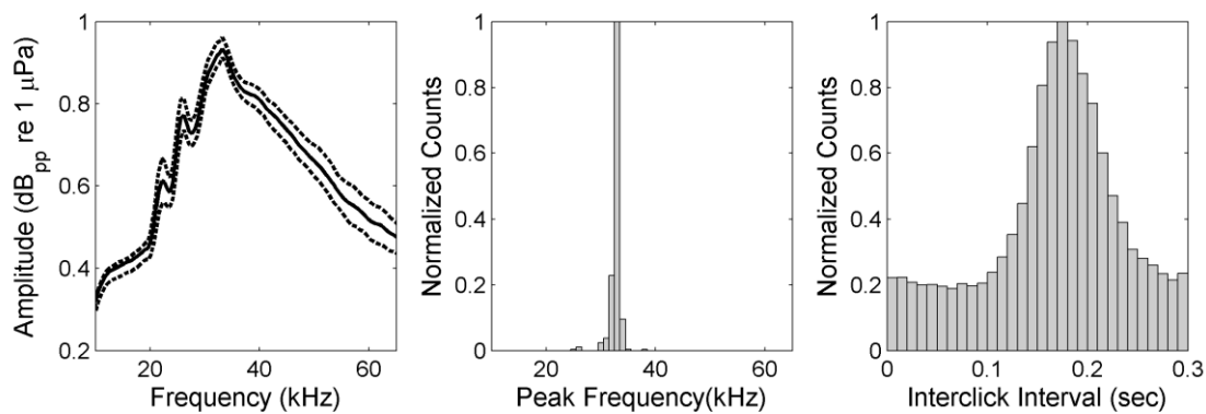
Figure 8. Risso's dolphin click type detected at site D from July to November 2015. Left: Mean frequency spectrum of click cluster (solid line) and 25 th and 75 th percentiles (dashed lines); Center: Distribution of click cluster peak frequencies; Right: Distribution of inter-click intervals (ICI) within cluster.
