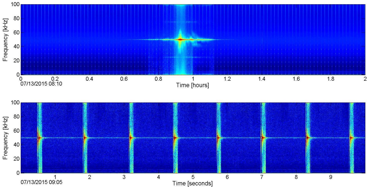
Figure 17. Echosounders in LTSA (top) and spectrogram (bottom) recorded at JAX site D in July 2015.
