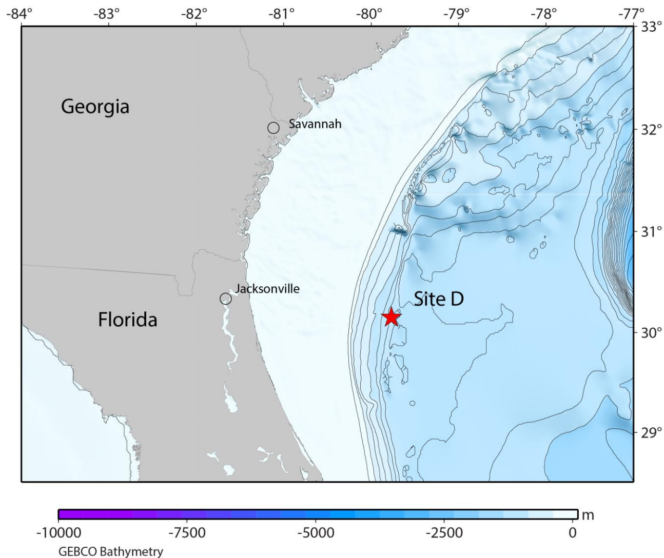
Figure 1. Location of High-frequency Acoustic Recording Package (HARP) at site D (30° 09.036 N, 79° 46.203 W, depth 800 m) deployed in the Jacksonville Range Complex study area from July to November 2015.
