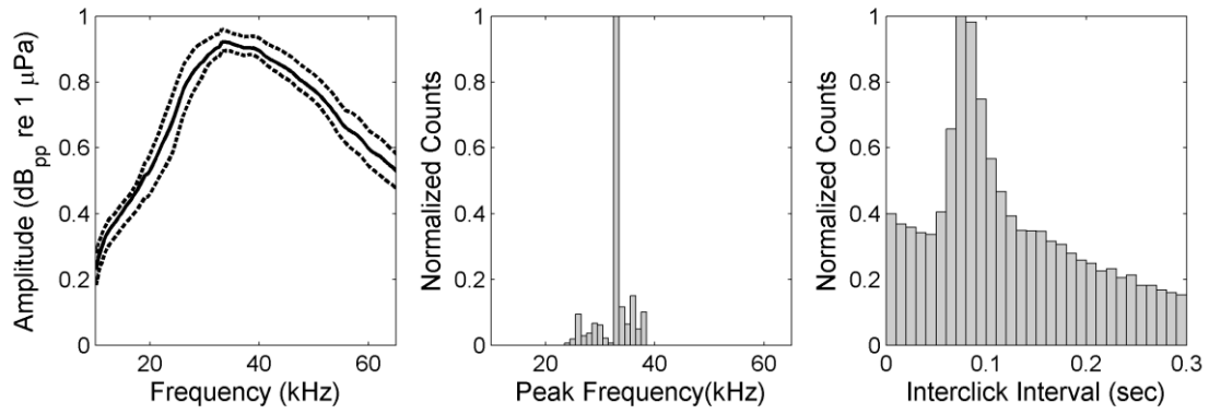
Figure 9. Click type CT J1 detected at JAX site D from July to November 2015. Left: Mean frequency spectrum of click cluster (solid line) and 25 th and 75 th percentiles (dashed lines); Center: Distribution of click cluster peak frequencies; Right: Distribution of inter-click intervals (ICI) within cluster.
