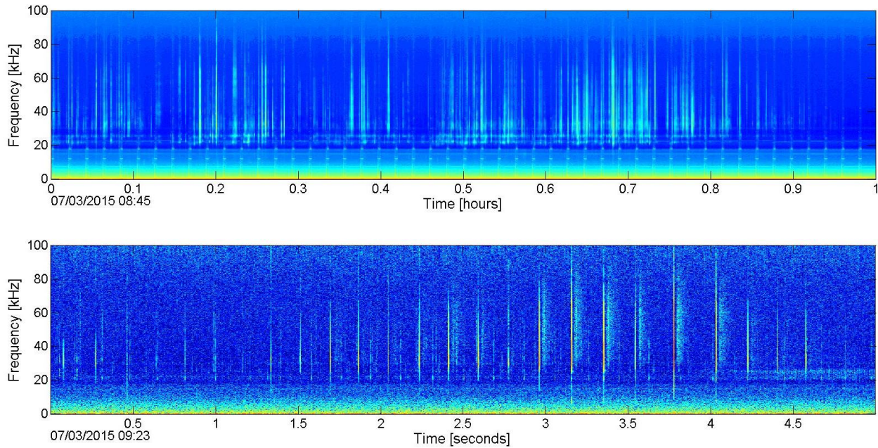
Figure 7. Risso's dolphin acoustic encounter in LTSA (top) and spectrogram (bottom) from HARP recording within the Jacksonville Range Complex, July 2015.
