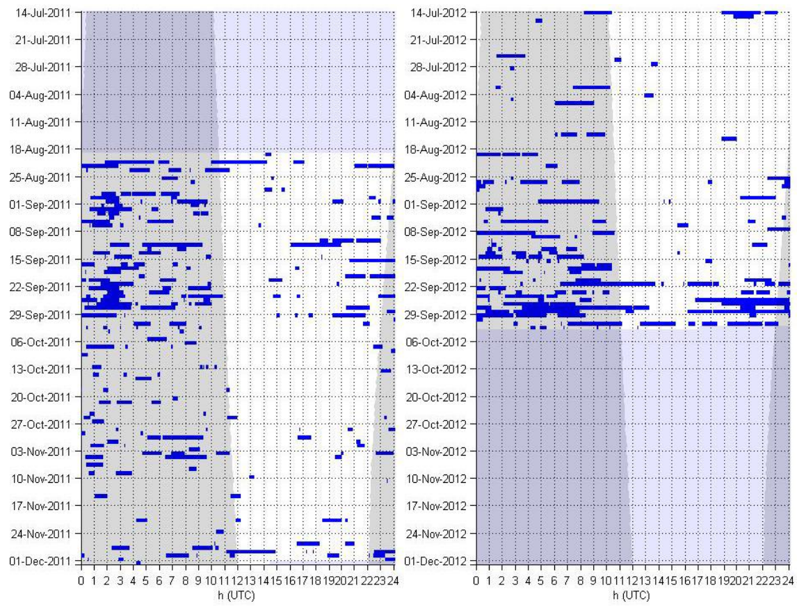
Unidentified odontocete whistles – Occurrence in 1 minute bins in 2011 (left) and 2012 (right).
