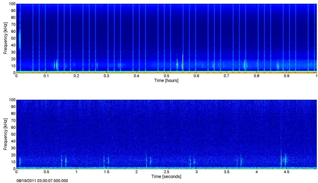
Figure 24. Sperm whale echolocation clicks in the LTSA (top) and spectrogram (bottom) from USWTR06E.
