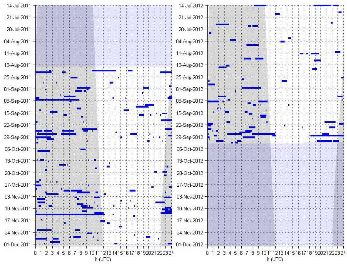
Unidentified odontocete clicks - Occurrence in 1 minute bins in 2011 (left) and 2012 (right).
