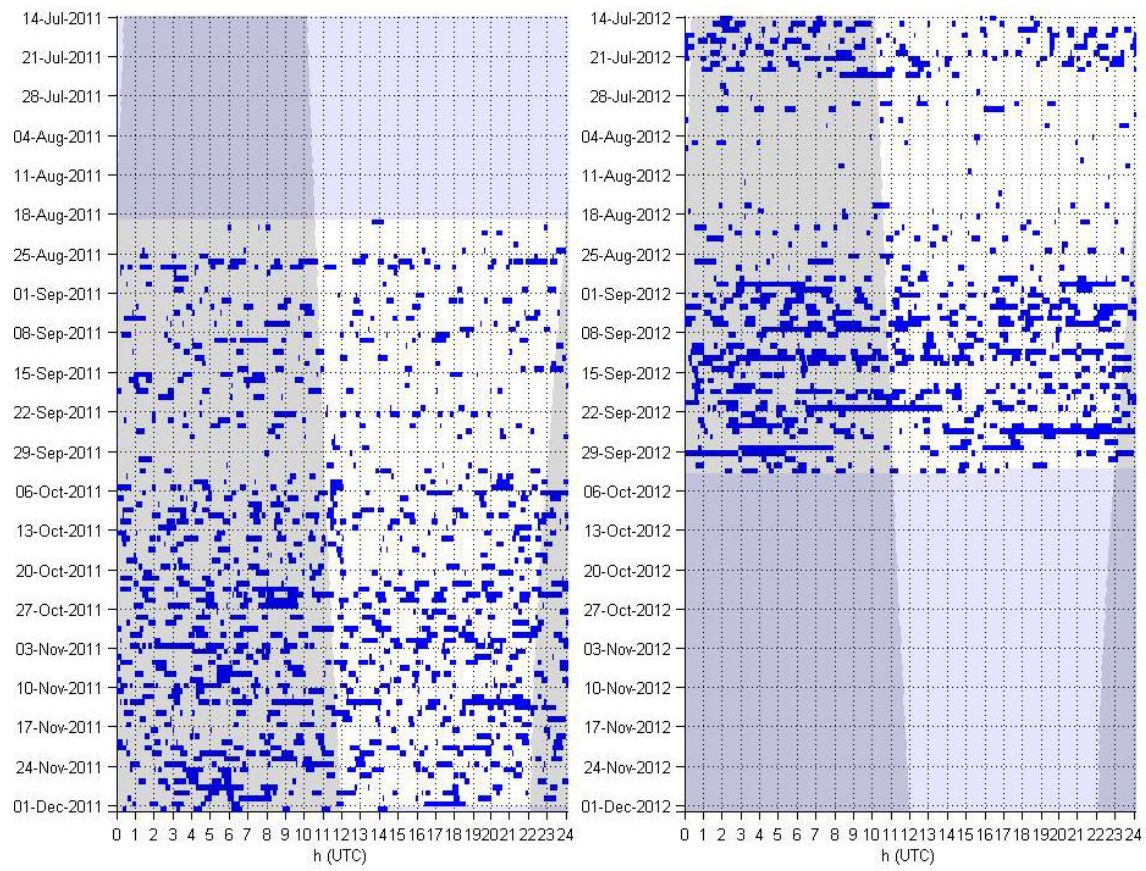
Gervais' beaked whales - Occurrence in 1 minute bins in 2011 (left) and 2012 (right).
