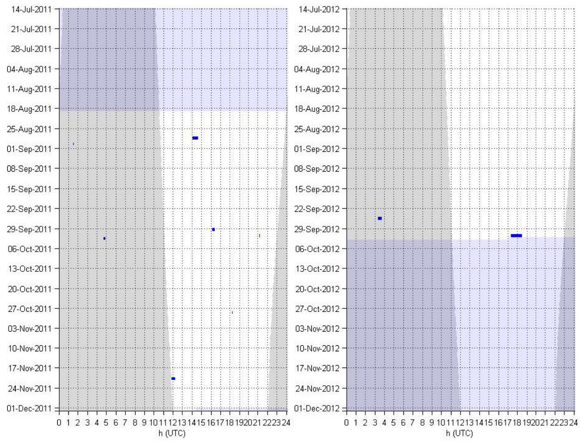
CT 26 – Occurrence in 1 minute bins in 2011 (left) and 2012 (right).
