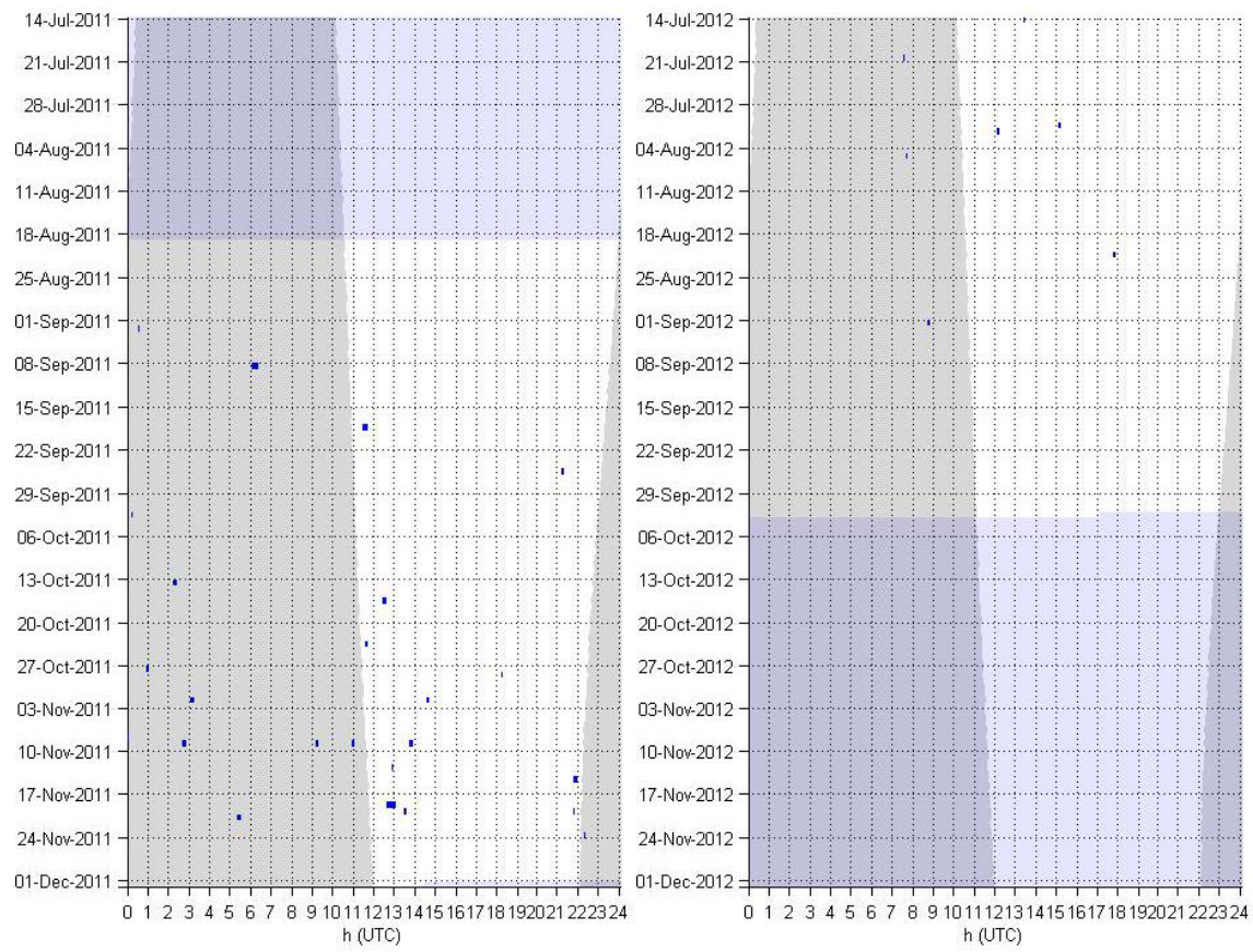
Kogia spp. - Occurrence in 1 minute bins in 2011 (left) and 2012 (right).
