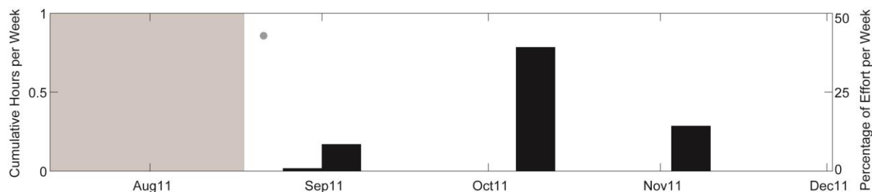
Figure 45. Weekly occurrence of BW38 calls in 2011. The area shaded in gray represents the section of data where there were no recordings. Recording effort was at 50% (5 minutes every 10 minutes). The light gray dots represent recording effort during partial weeks.
