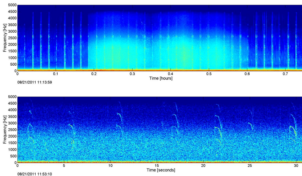
Figure 13. Unidentified odontocete whistles <5 kHz from USWTR06E.
