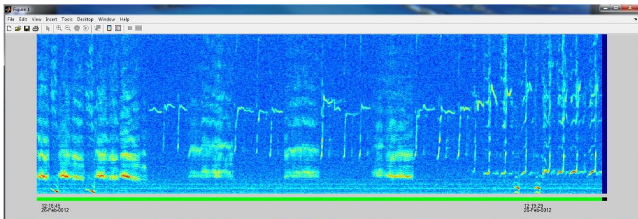
Figure 12. Example of humpback whale song from southern California in analyst verification stage of detector.
