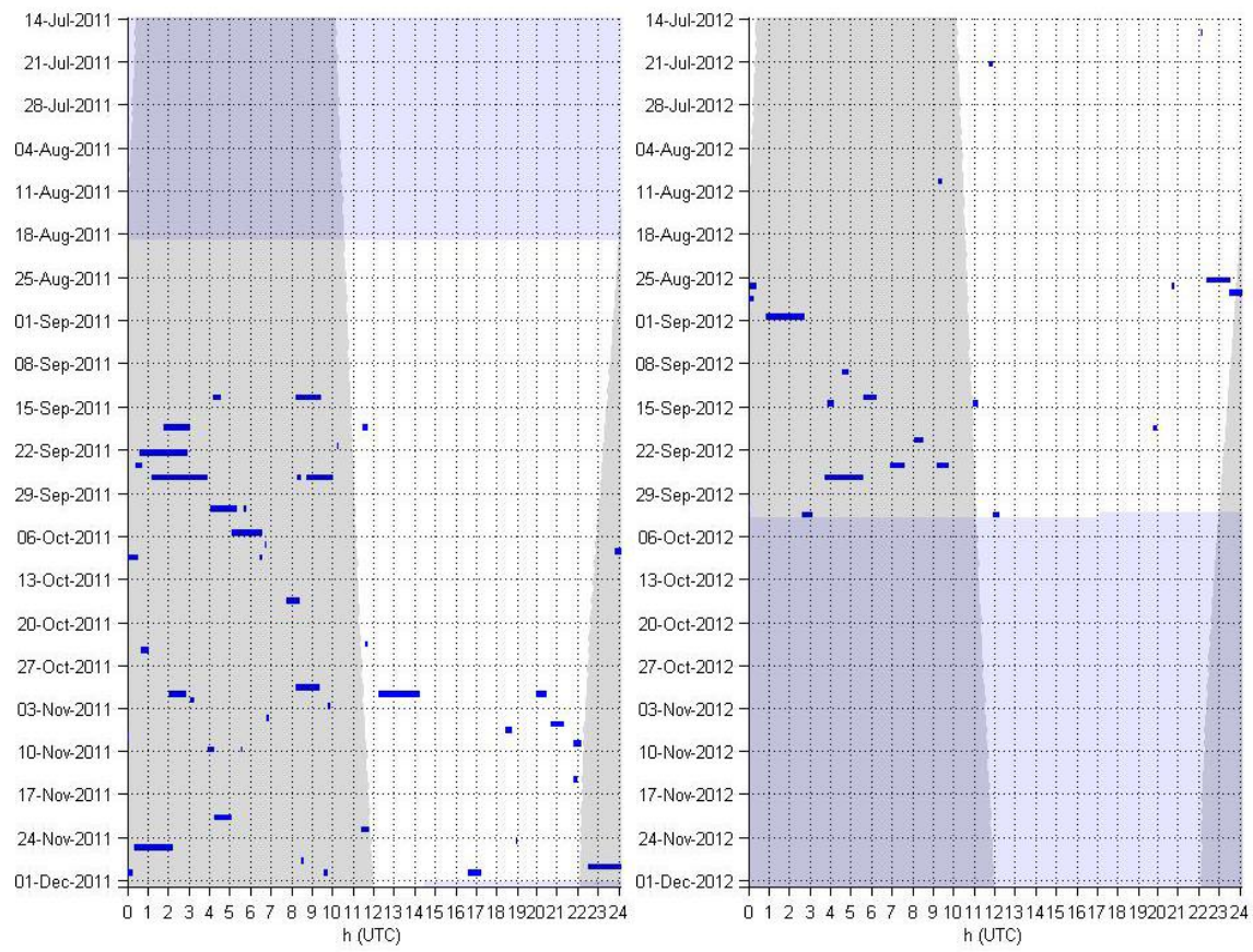
CT 32 – Occurrence in 1 minute bins in 2011 (left) and 2012 (right).
