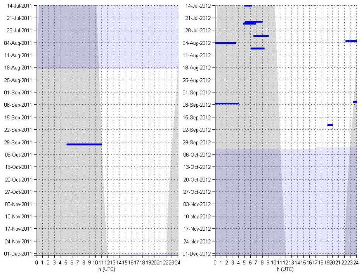
Risso's dolphins - Occurrence in 1 minute bins in 2011 (left) and 2012 (right).
