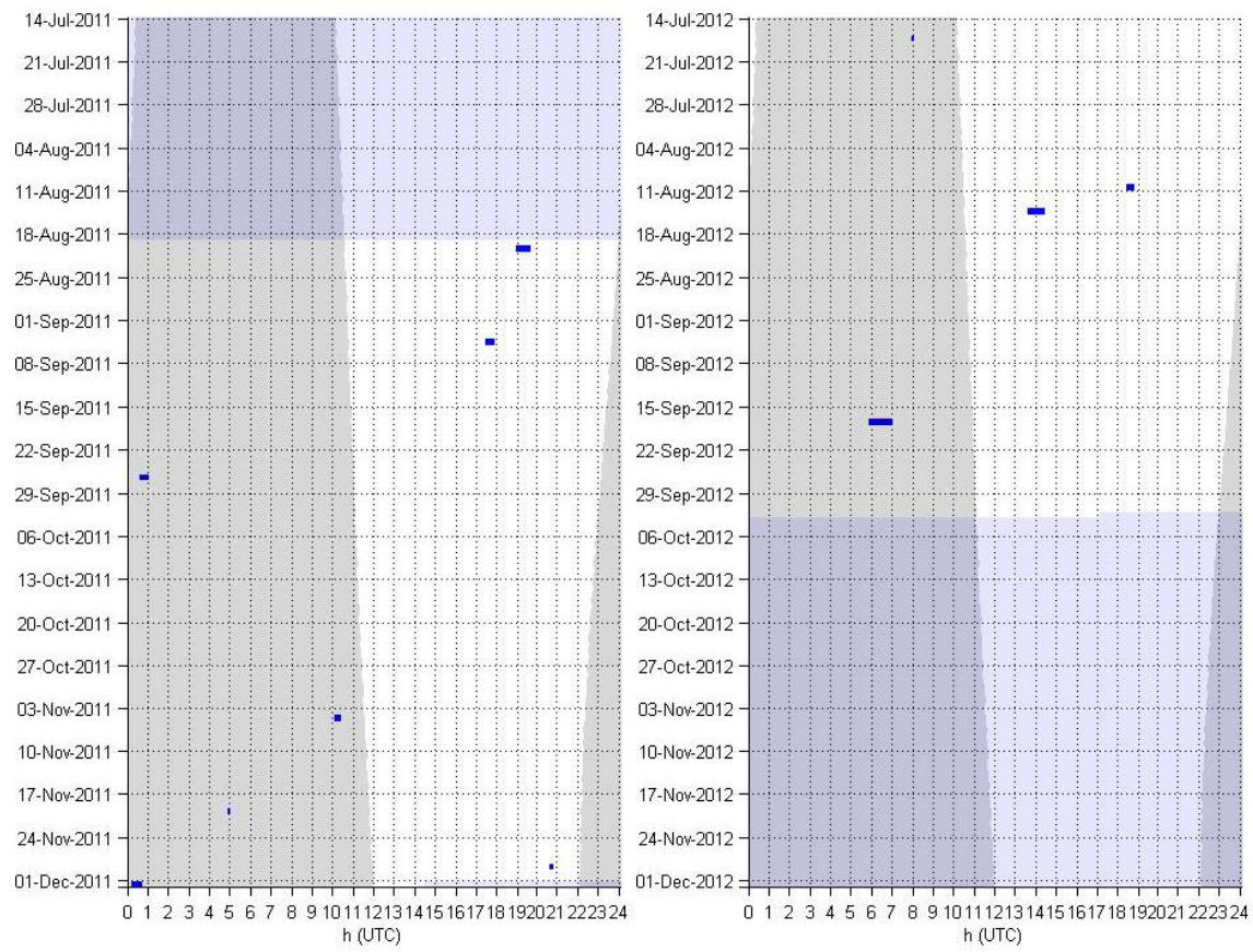
Echosounders – Occurrence in 1 minute bins in 2011 (left) and 2012 (right).
