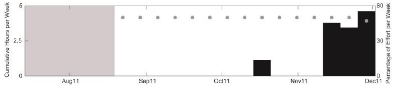
Figure 44. Weekly occurrence of downsweep calls in 2011. Effort as described in Figure 42.
