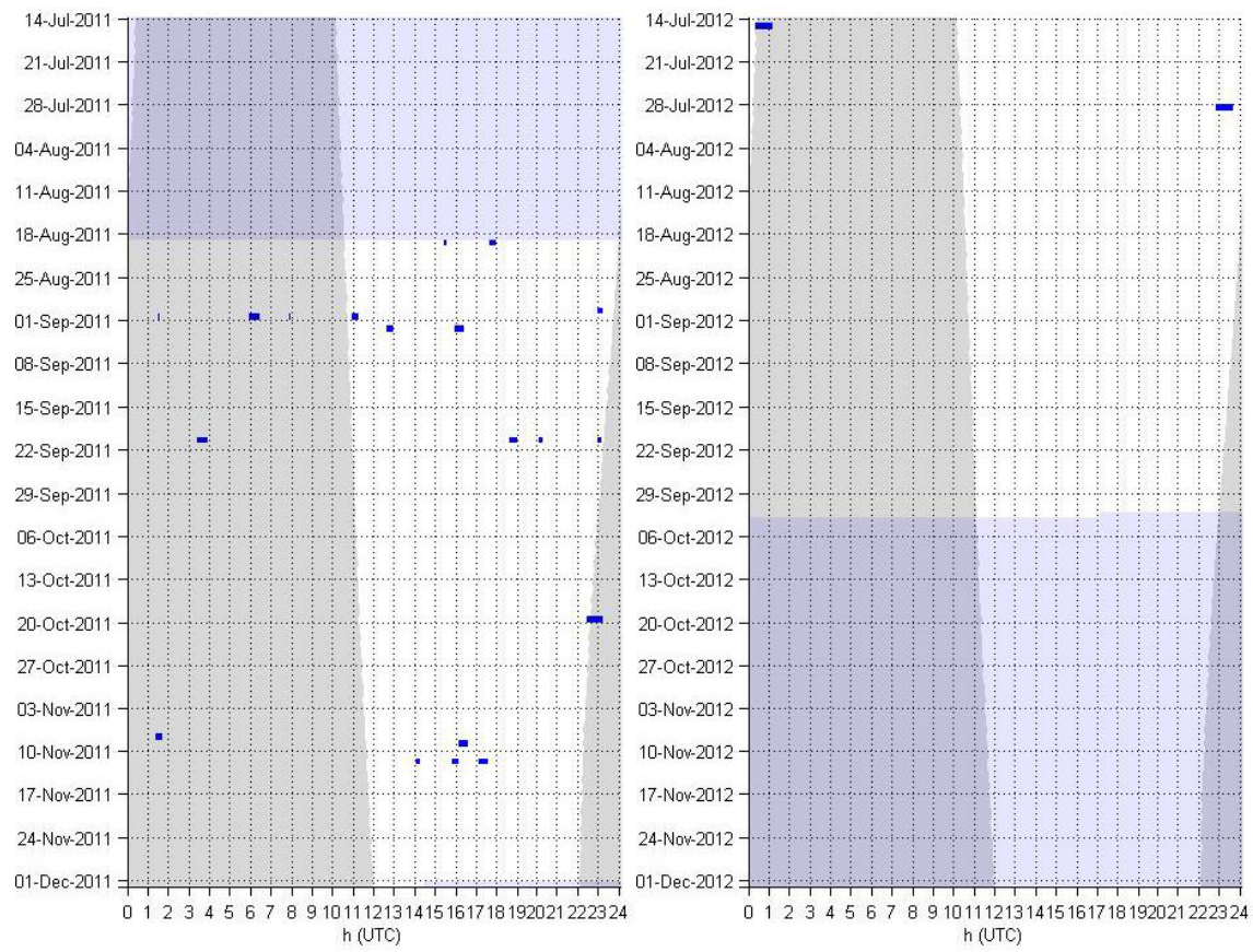
Blainville's beaked whales - Occurrence in 1 minute bins in 2011 (left) and 2012 (right).
