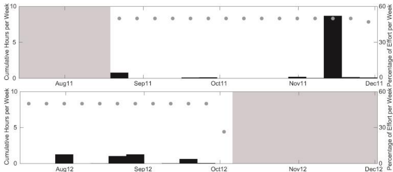
Figure 51. Weekly unidentified odontocete whistles <5 kHz presence in 2011 (top) and 2012 (bottom). Effort as described in Figure 45.
