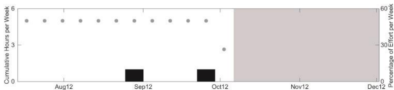
Figure 41. Weekly blue whale call presence in 2012. Effort is as described in Figure 40.
