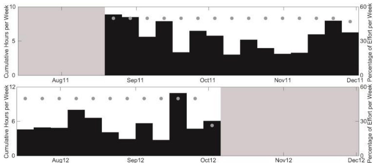
Figure 60. Weekly broadband ship noise in 2011 (top) and 2012 (bottom). The area shaded in gray represents where there were no recordings. The light gray dots represent weekly recording effort.
