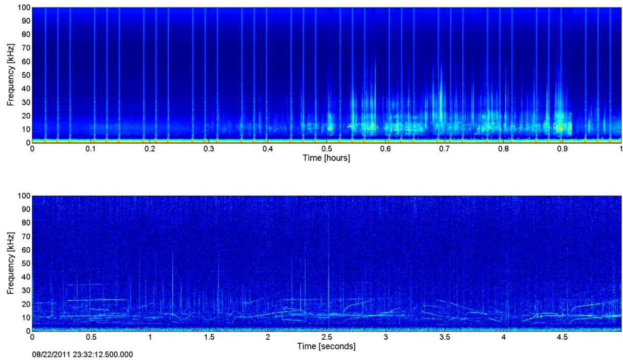
Figure 20. LTSA (top) and spectrogram (bottom) of odontocete echolocation clicks and whistles from USWTR06E.
