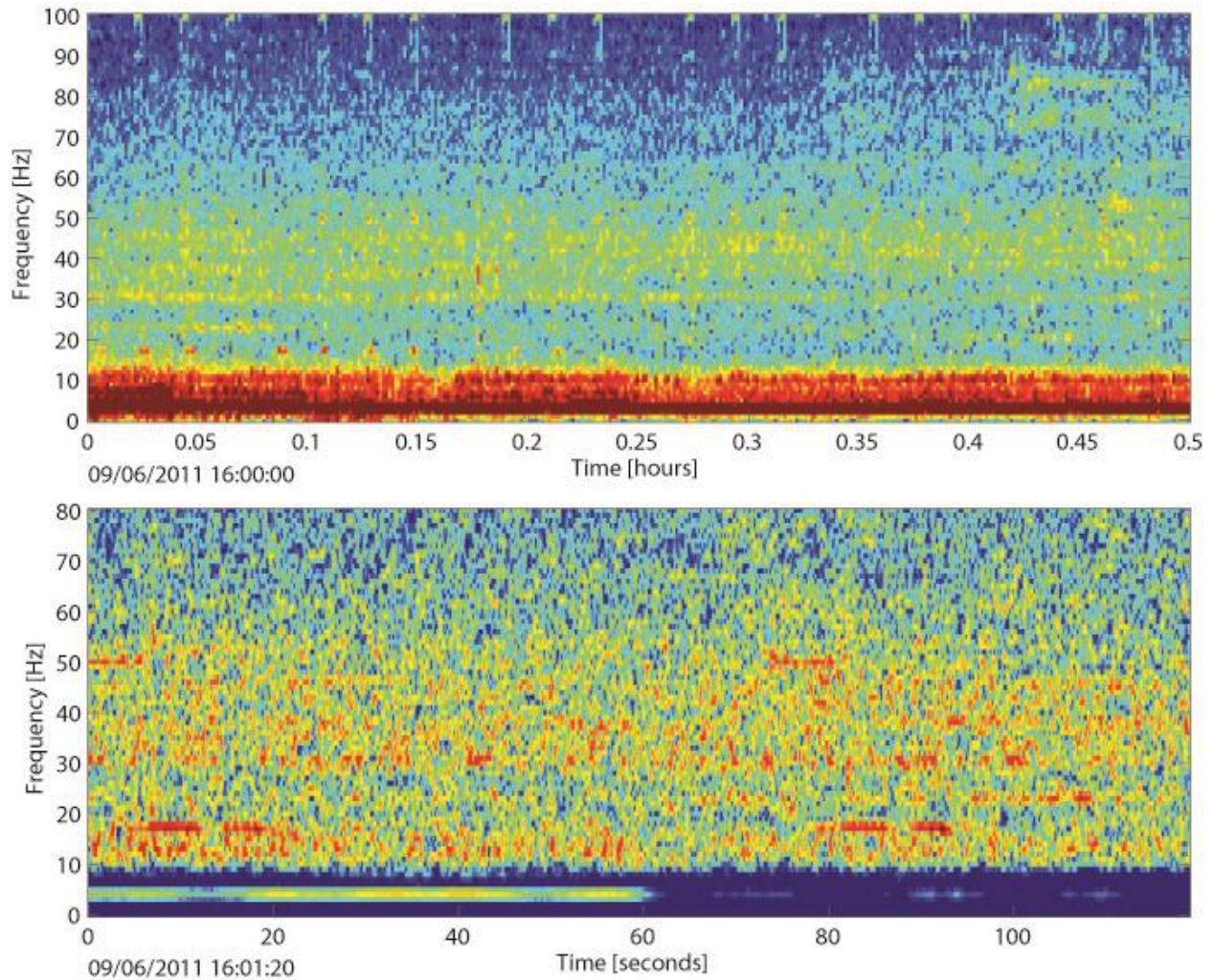
Figure 3. Blue whale calls in the LTSA (top) and spectrogram (bottom) from the USWTR data.
