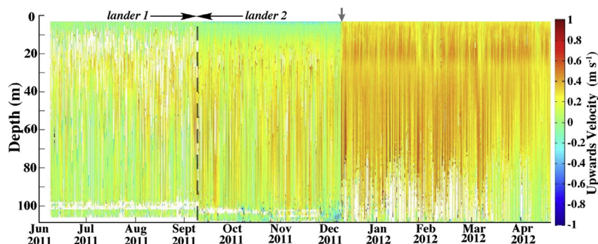
Figure 8. Upwelling velocity from ADCP data for both deployments. Velocities restricted to the range -1 to 1 \text{ m s}^{-1} with scale on right. White regions are data blanked from bubble contamination. Downward arrow indicates 8 December 2011 event, and dotted line delineates the two lander deployments.
